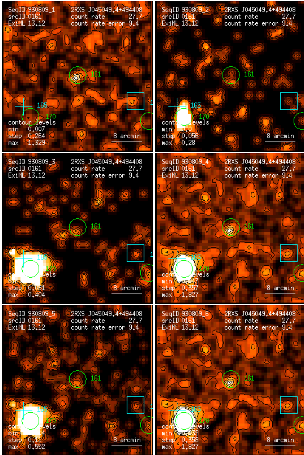
Figure 161: RASS 930809: detection 0161: band rate images, Gaussian filter: (1) PSPC channels 11 – 41, (2) 52 – 90, (3) 91 – 201, (4) 11 – 235, (5) 52 – 201, (6) 11 – 201. Broad band rates in counts/ks. Band rate contour levels in counts/ks/arcmin 2 .
