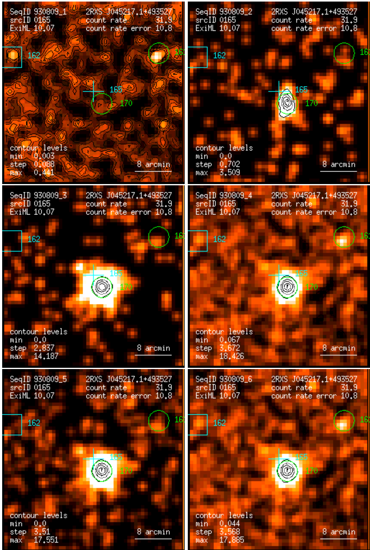
Figure 165: RASS 930809: detection 0165: band rate images, Gaussian filter: (1) PSPC channels 11 – 41, (2) 52 – 90, (3) 91 – 201, (4) 11 – 235, (5) 52 – 201, (6) 11 – 201. Broad band rates in counts/ks. Band rate contour levels in counts/ks/arcmin 2 .
