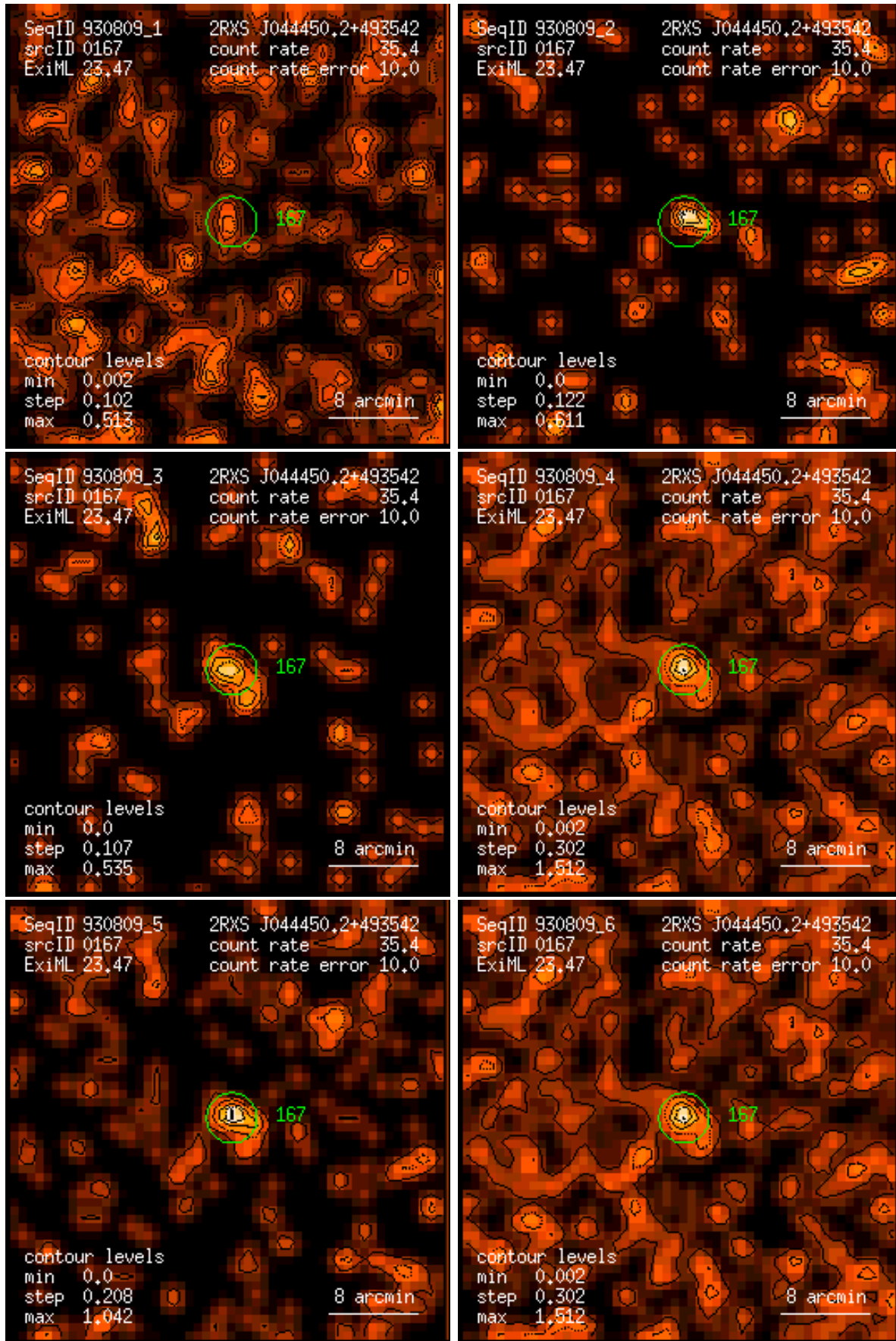
Figure 167: RASS 930809: detection 0167: band rate images, Gaussian filter: (1) PSPC channels 11 – 41, (2) 52 – 90, (3) 91 – 201, (4) 11 – 235, (5) 52 – 201, (6) 11 – 201. Broad band rates in counts/ks. Band rate contour levels in counts/ks/arcmin 2 .
