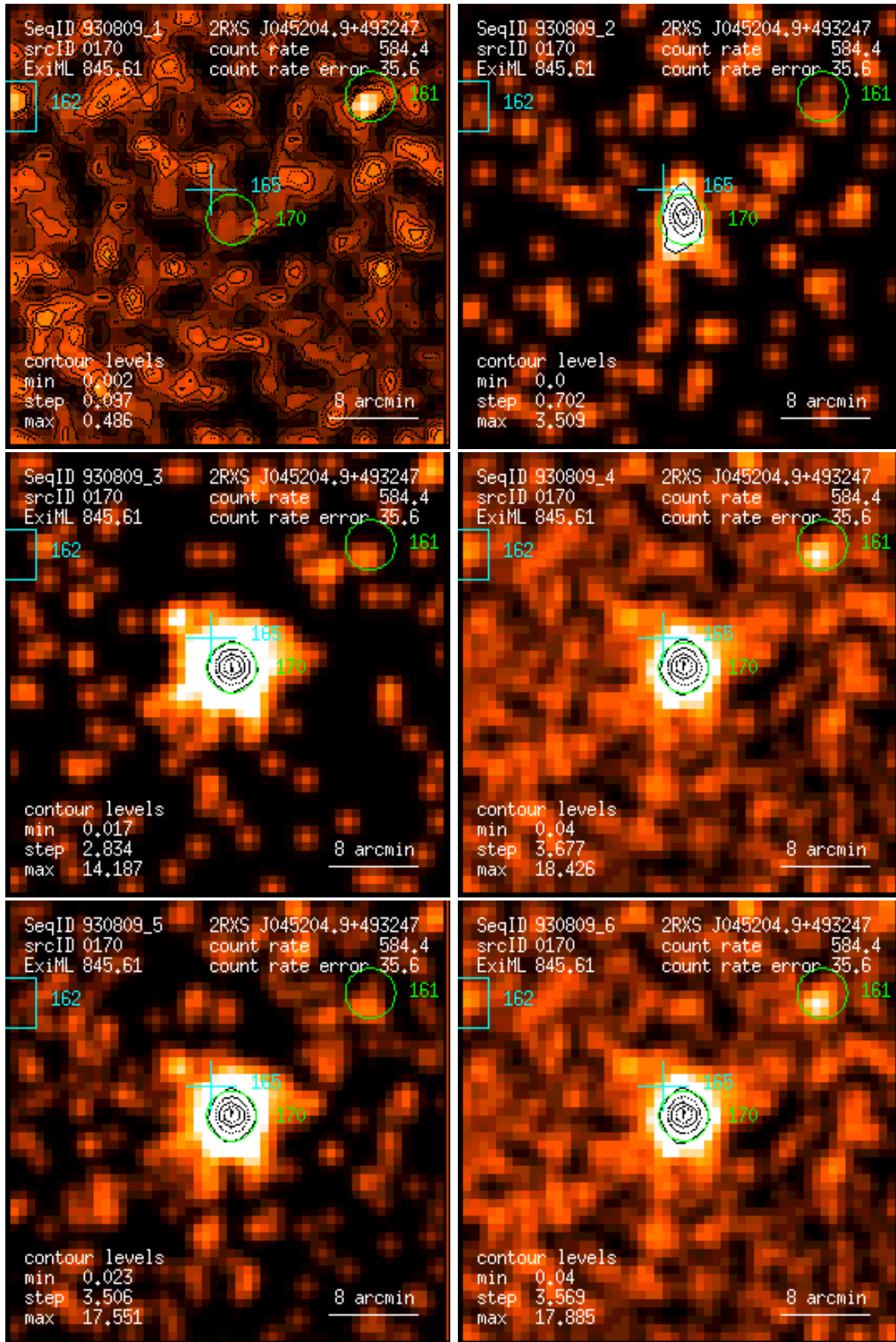
Figure 170: RASS 930809: detection 0170: band rate images, Gaussian filter: (1) PSPC channels 11 – 41, (2) 52 – 90, (3) 91 – 201, (4) 11 – 235, (5) 52 – 201, (6) 11 – 201. Broad band rates in counts/ks. Band rate contour levels in counts/ks/arcmin 2 .
