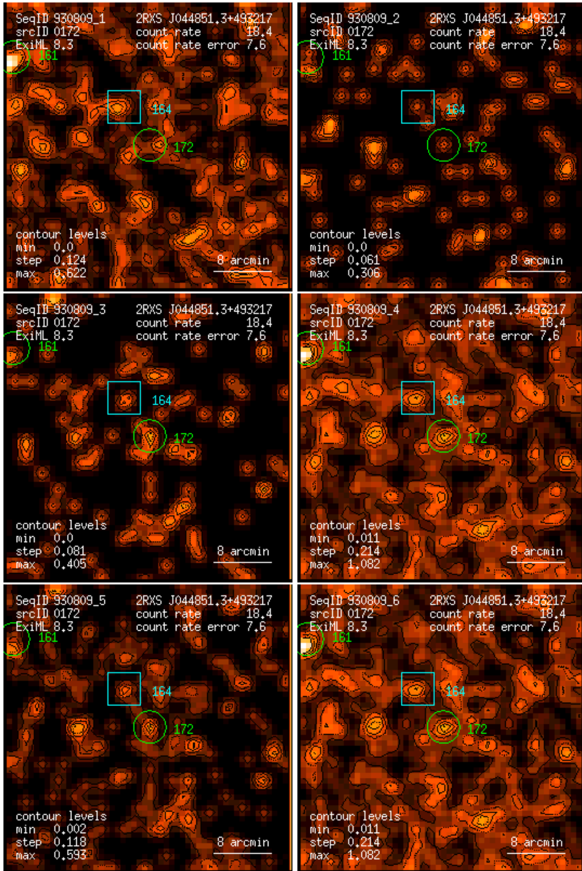
Figure 172: RASS 930809: detection 0172: band rate images, Gaussian filter: (1) PSPC channels 11 – 41, (2) 52 – 90, (3) 91 – 201, (4) 11 – 235, (5) 52 – 201, (6) 11 – 201. Broad band rates in counts/ks. Band rate contour levels in counts/ks/arcmin 2 .
