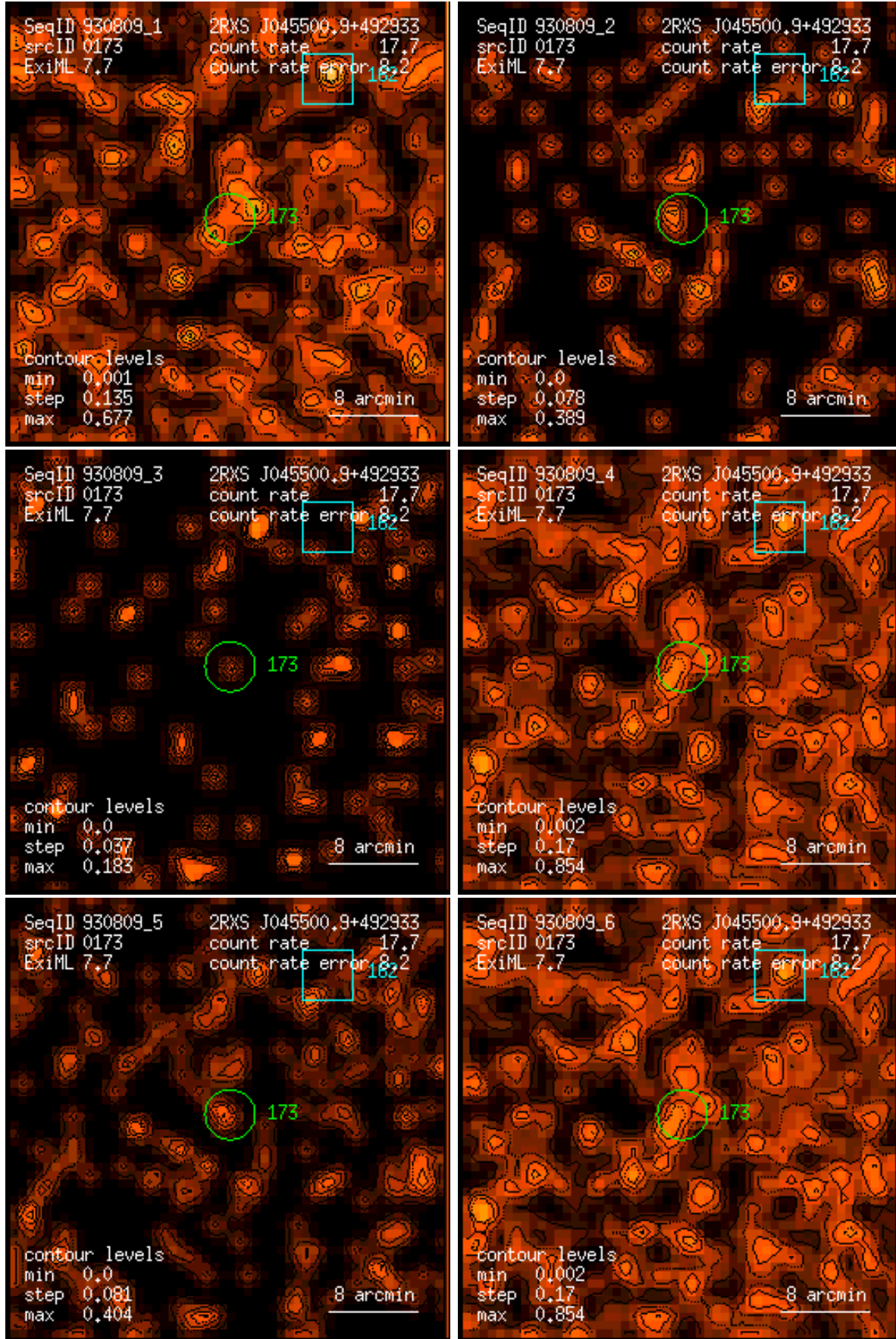
Figure 173: RASS 930809: detection 0173: band rate images, Gaussian filter: (1) PSPC channels 11 – 41, (2) 52 – 90, (3) 91 – 201, (4) 11 – 235, (5) 52 – 201, (6) 11 – 201. Broad band rates in counts/ks. Band rate contour levels in counts/ks/arcmin 2 .
