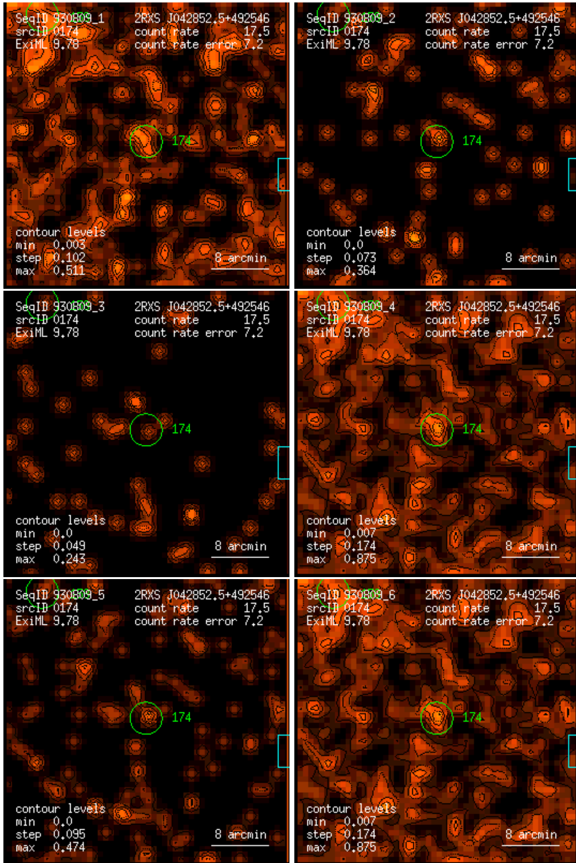
Figure 174: RASS 930809: detection 0174: band rate images, Gaussian filter: (1) PSPC channels 11 – 41, (2) 52 – 90, (3) 91 – 201, (4) 11 – 235, (5) 52 – 201, (6) 11 – 201. Broad band rates in counts/ks. Band rate contour levels in counts/ks/arcmin 2 .
