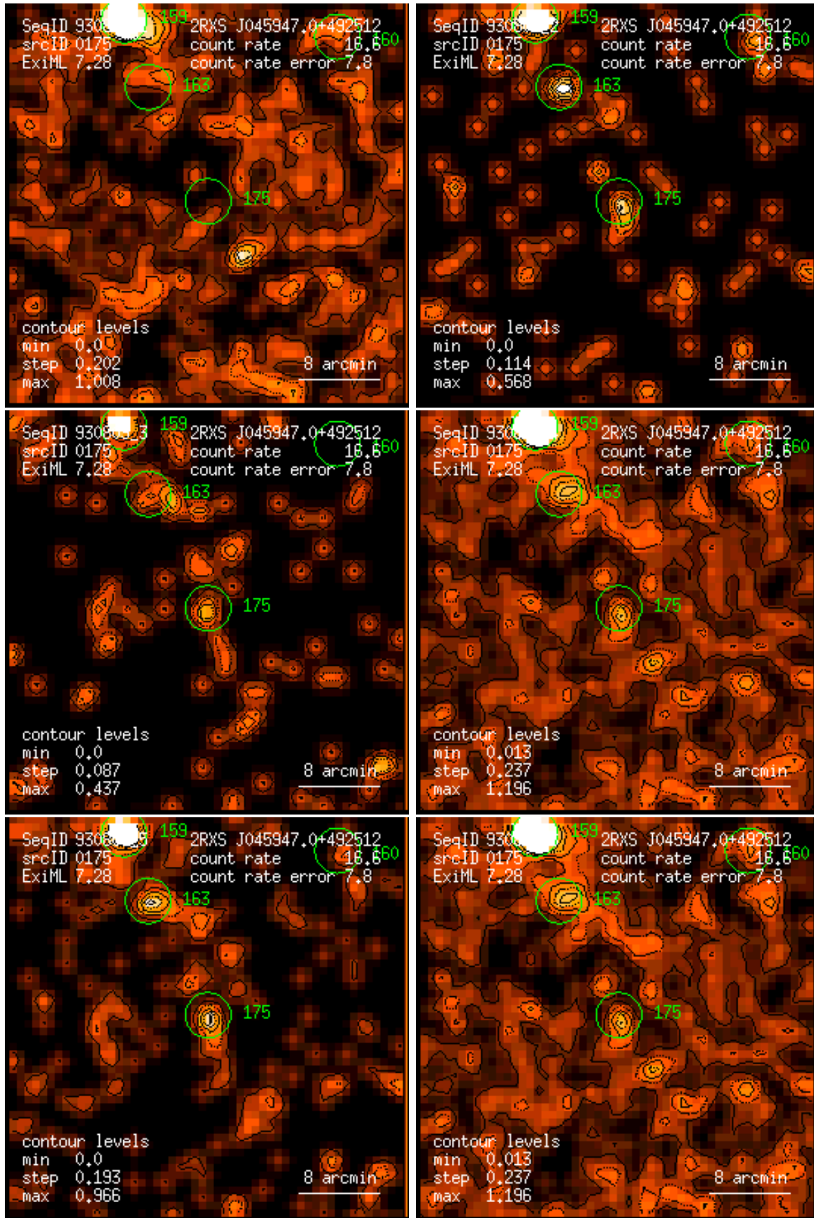
Figure 175: RASS 930809: detection 0175: band rate images, Gaussian filter: (1) PSPC channels 11 – 41, (2) 52 – 90, (3) 91 – 201, (4) 11 – 235, (5) 52 – 201, (6) 11 – 201. Broad band rates in counts/ks. Band rate contour levels in counts/ks/arcmin 2 .
