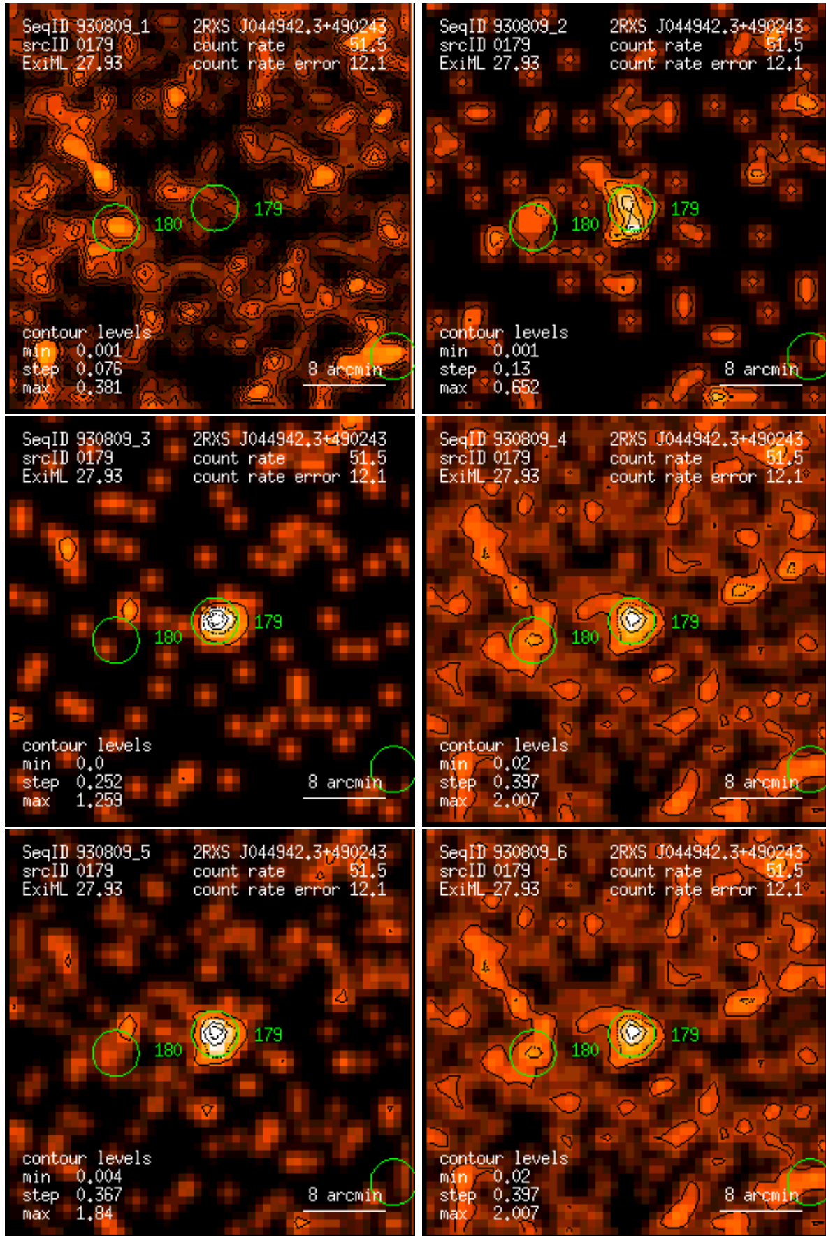
Figure 179: RASS 930809: detection 0179: band rate images, Gaussian filter: (1) PSPC channels 11 – 41, (2) 52 – 90, (3) 91 – 201, (4) 11 – 235, (5) 52 – 201, (6) 11 – 201. Broad band rates in counts/ks. Band rate contour levels in counts/ks/arcmin 2 .
