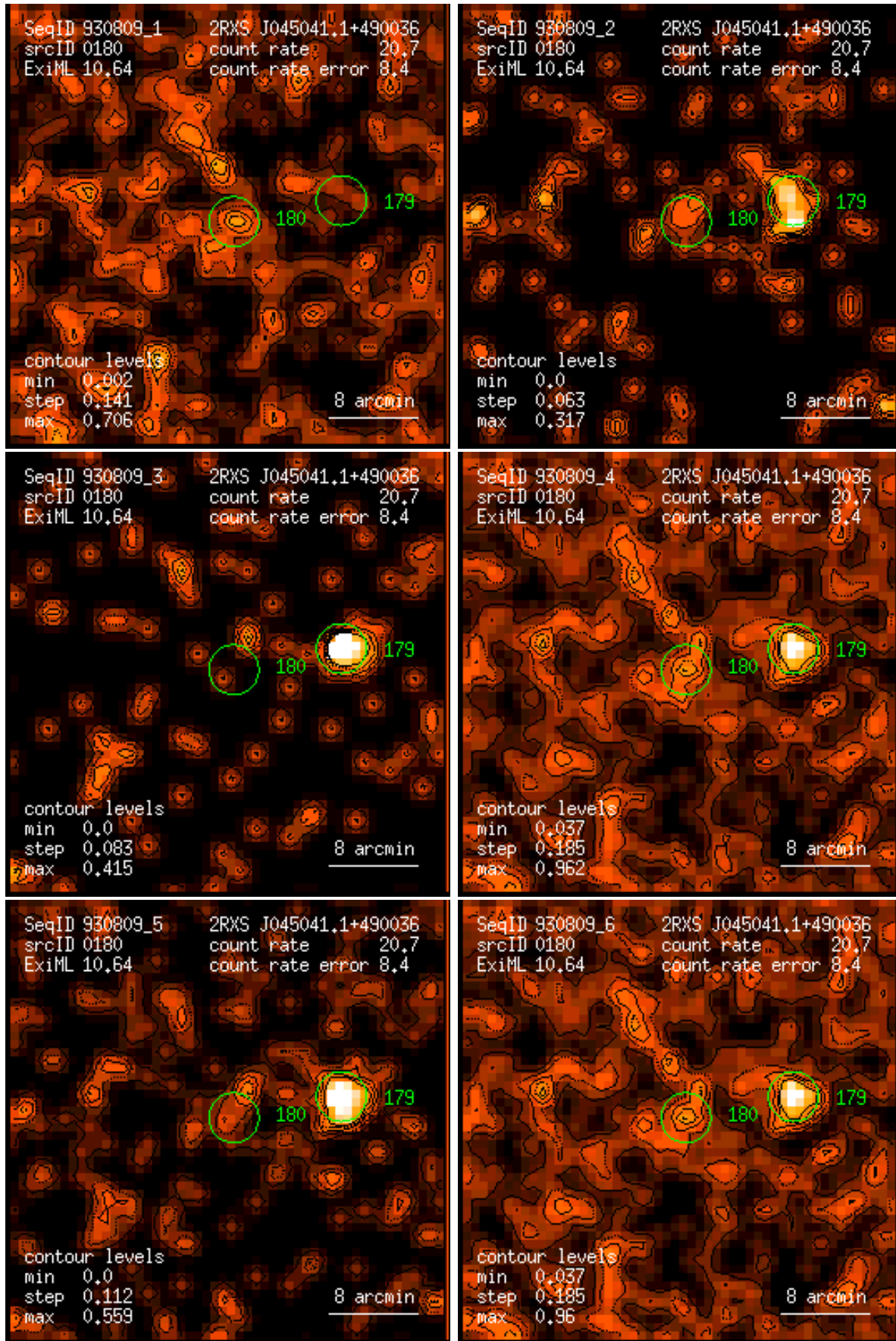
Figure 180: RASS 930809: detection 0180: band rate images, Gaussian filter: (1) PSPC channels 11 – 41, (2) 52 – 90, (3) 91 – 201, (4) 11 – 235, (5) 52 – 201, (6) 11 – 201. Broad band rates in counts/ks. Band rate contour levels in counts/ks/arcmin 2 .
