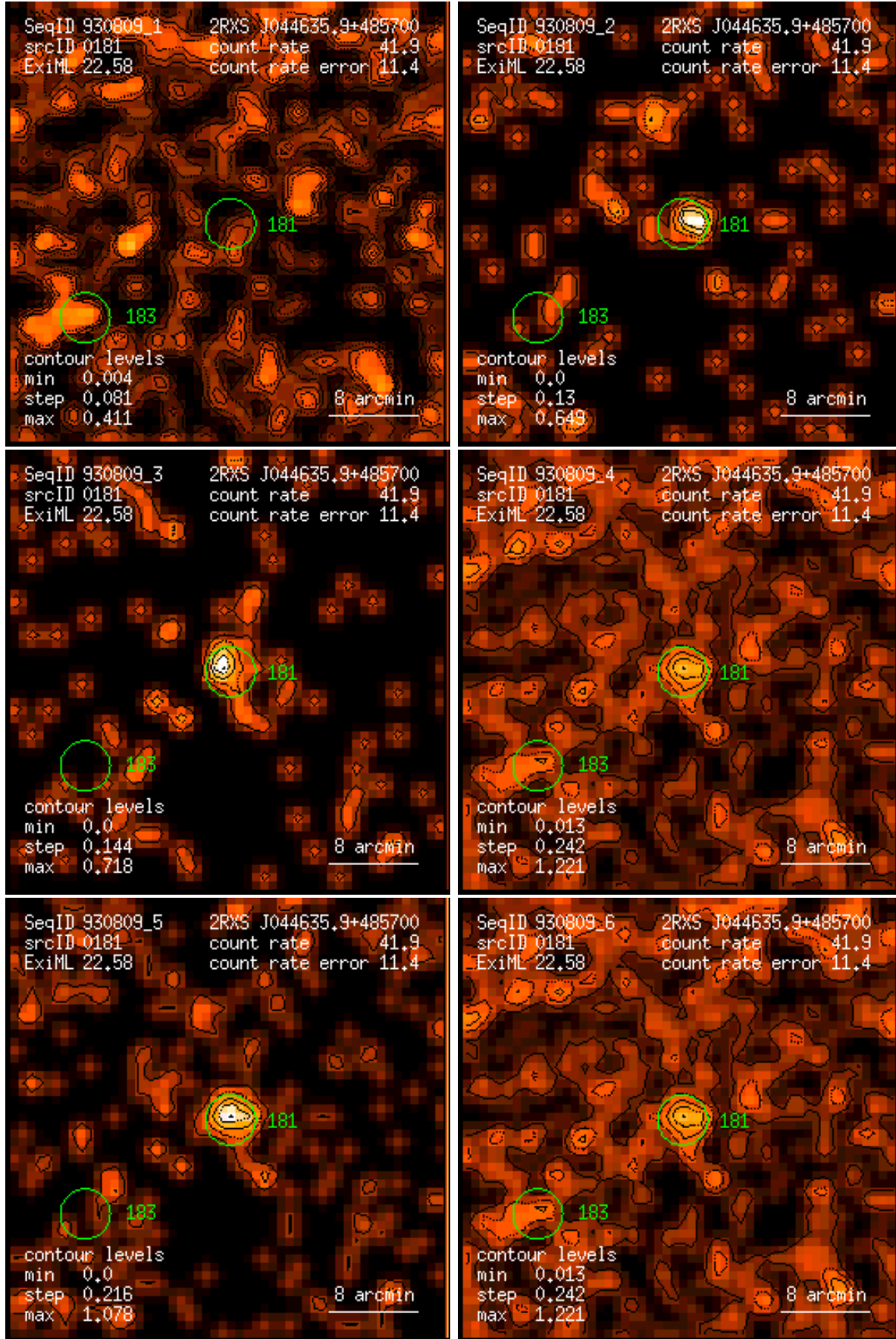
Figure 181: RASS 930809: detection 0181: band rate images, Gaussian filter: (1) PSPC channels 11 – 41, (2) 52 – 90, (3) 91 – 201, (4) 11 – 235, (5) 52 – 201, (6) 11 – 201. Broad band rates in counts/ks. Band rate contour levels in counts/ks/arcmin 2 .
