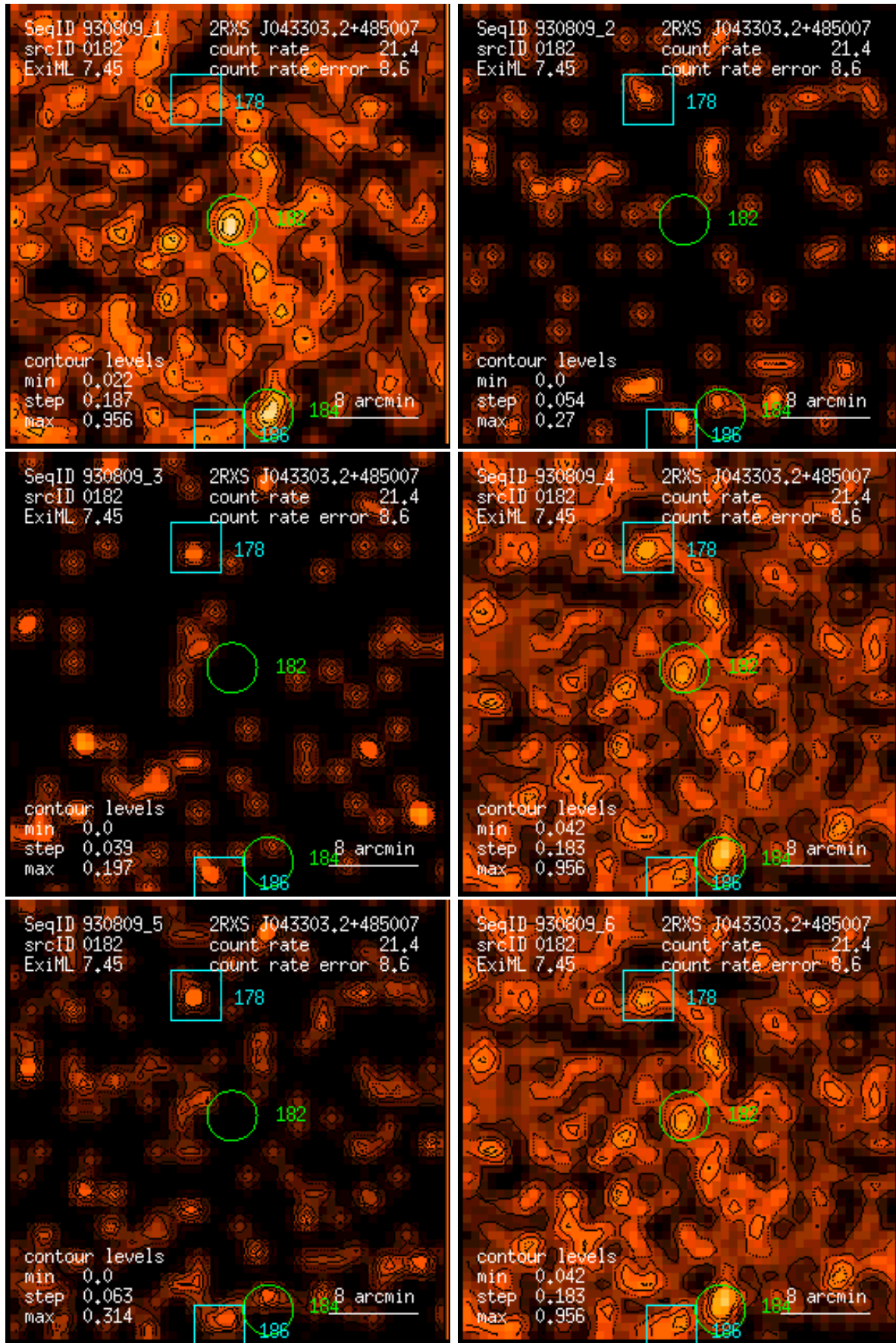
Figure 182: RASS 930809: detection 0182: band rate images, Gaussian filter: (1) PSPC channels 11 – 41, (2) 52 – 90, (3) 91 – 201, (4) 11 – 235, (5) 52 – 201, (6) 11 – 201. Broad band rates in counts/ks. Band rate contour levels in counts/ks/arcmin 2 .
