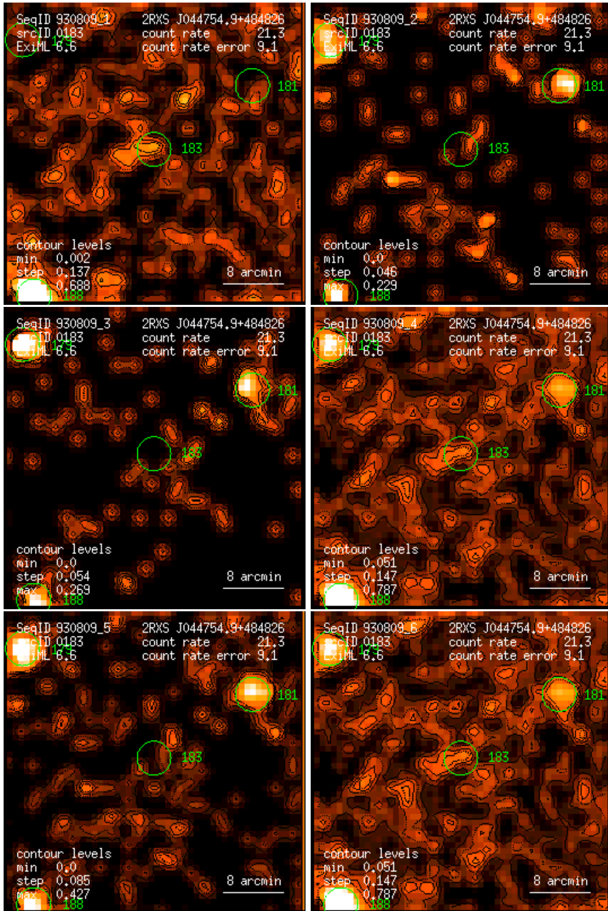
Figure 183: RASS 930809: detection 0183: band rate images, Gaussian filter: (1) PSPC channels 11 – 41, (2) 52 – 90, (3) 91 – 201, (4) 11 – 235, (5) 52 – 201, (6) 11 – 201. Broad band rates in counts/ks. Band rate contour levels in counts/ks/arcmin 2 .
