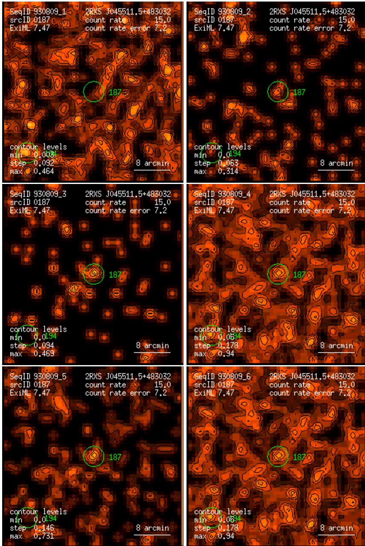
Figure 187: RASS 930809: detection 0187: band rate images, Gaussian filter: (1) PSPC channels 11 – 41, (2) 52 – 90, (3) 91 – 201, (4) 11 – 235, (5) 52 – 201, (6) 11 – 201. Broad band rates in counts/ks. Band rate contour levels in counts/ks/arcmin 2 .
