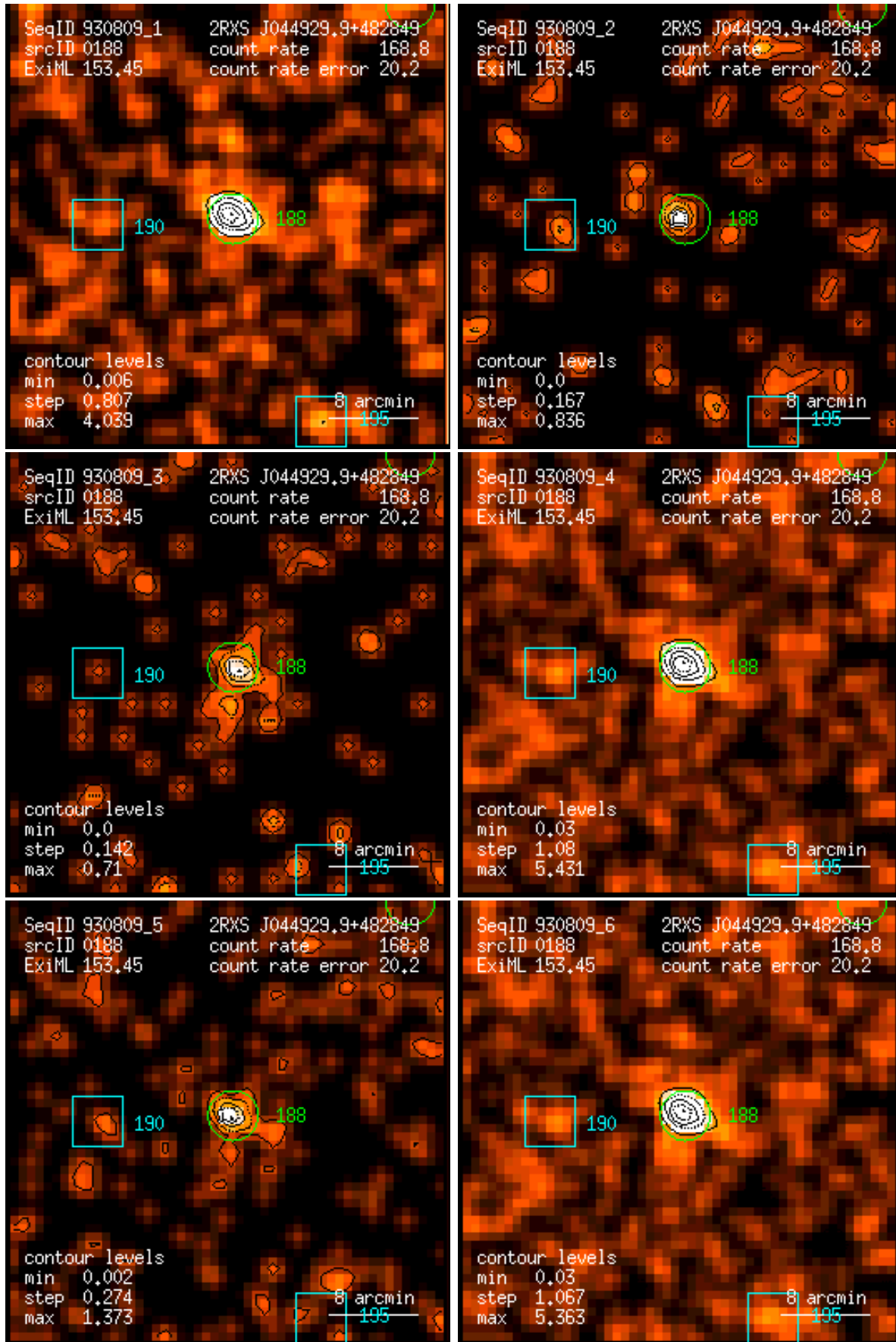
Figure 188: RASS 930809: detection 0188: band rate images, Gaussian filter: (1) PSPC channels 11 – 41, (2) 52 – 90, (3) 91 – 201, (4) 11 – 235, (5) 52 – 201, (6) 11 – 201. Broad band rates in counts/ks. Band rate contour levels in counts/ks/arcmin 2 .
