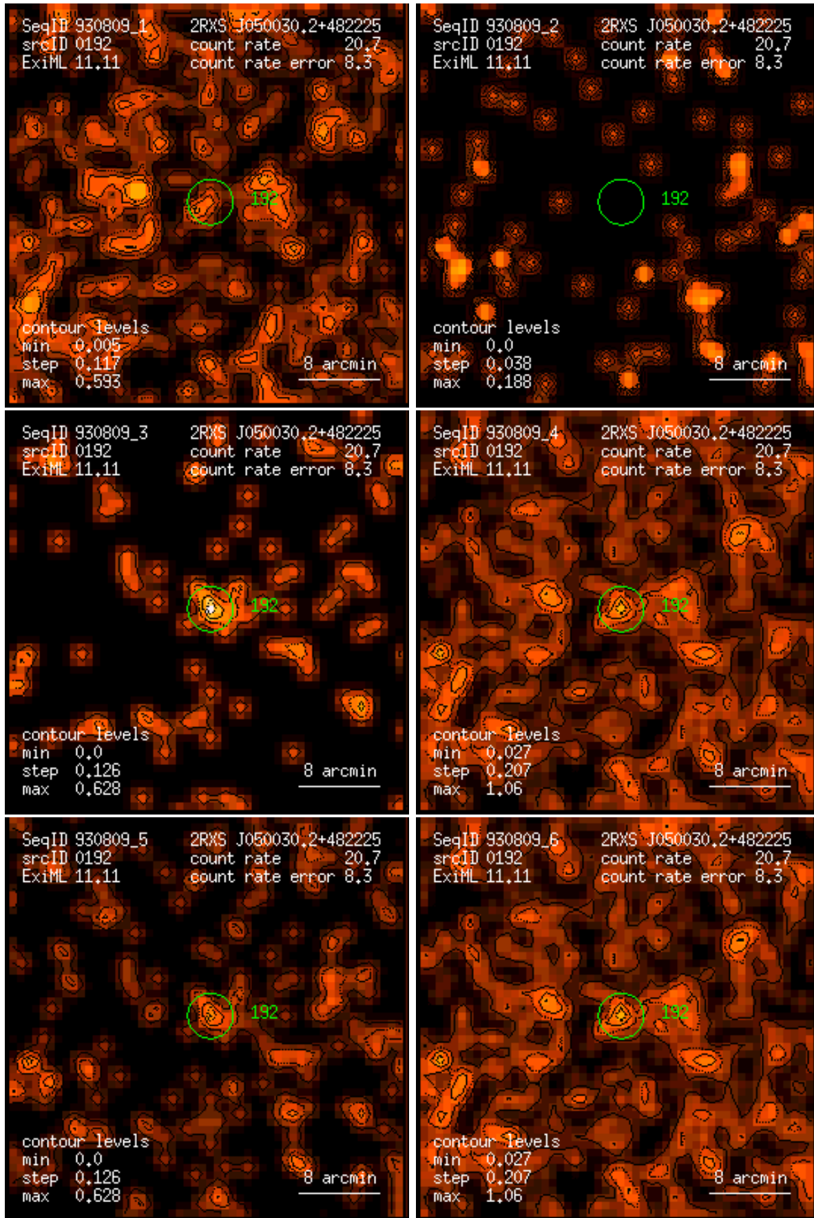
Figure 192: RASS 930809: detection 0192: band rate images, Gaussian filter: (1) PSPC channels 11 – 41, (2) 52 – 90, (3) 91 – 201, (4) 11 – 235, (5) 52 – 201, (6) 11 – 201. Broad band rates in counts/ks. Band rate contour levels in counts/ks/arcmin 2 .
