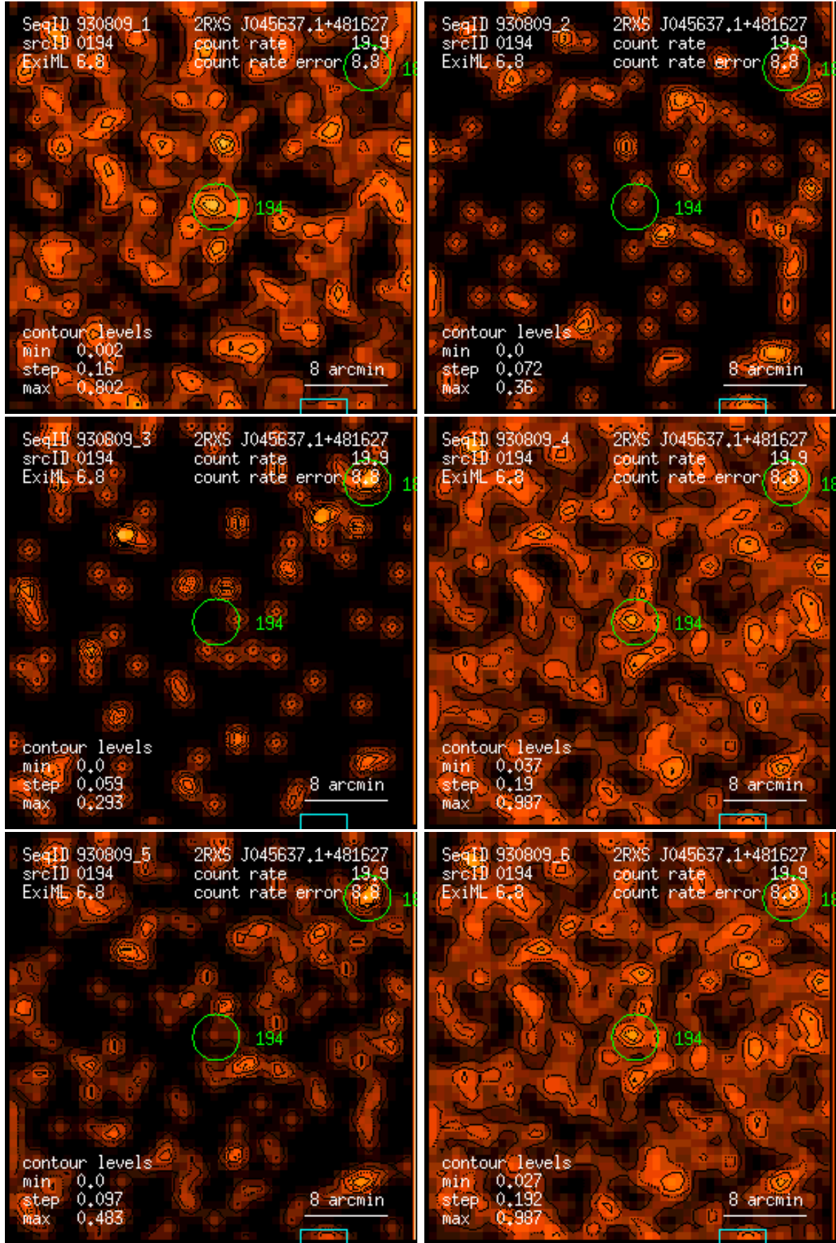
Figure 194: RASS 930809: detection 0194: band rate images, Gaussian filter: (1) PSPC channels 11 – 41, (2) 52 – 90, (3) 91 – 201, (4) 11 – 235, (5) 52 – 201, (6) 11 – 201. Broad band rates in counts/ks. Band rate contour levels in counts/ks/arcmin 2 .
