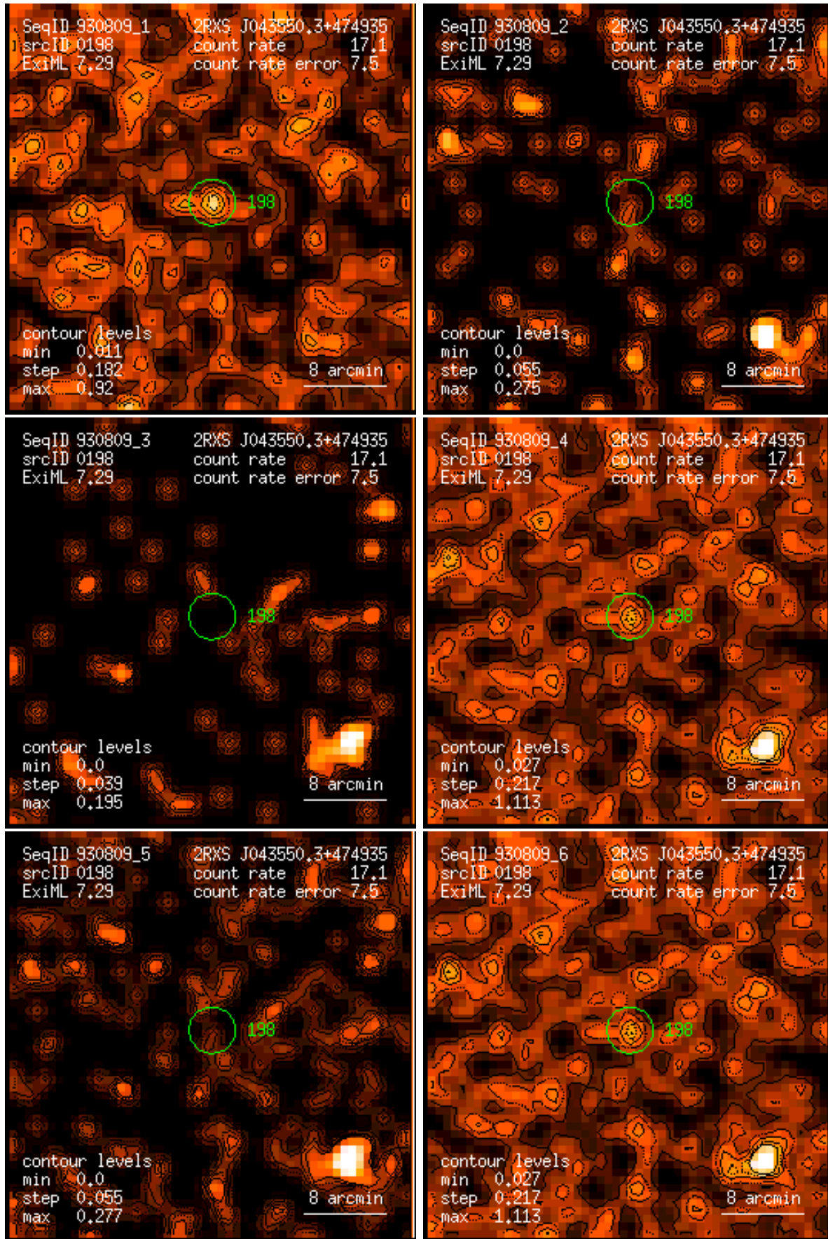
Figure 198: RASS 930809: detection 0198: band rate images, Gaussian filter: (1) PSPC channels 11 – 41, (2) 52 – 90, (3) 91 – 201, (4) 11 – 235, (5) 52 – 201, (6) 11 – 201. Broad band rates in counts/ks. Band rate contour levels in counts/ks/arcmin 2 .
