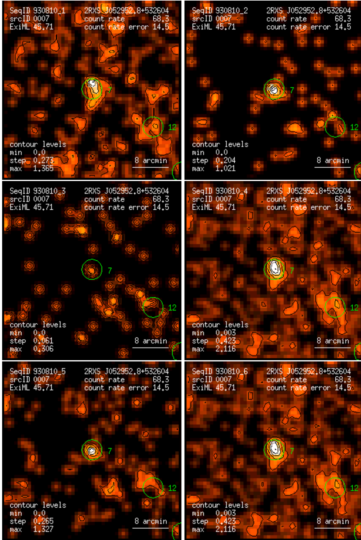
Figure 7: RASS 930810: detection 0007: band rate images, Gaussian filter: (1) PSPC channels 11 – 41, (2) 52 – 90, (3) 91 – 201, (4) 11 – 235, (5) 52 – 201, (6) 11 – 201. Broad band rates in counts/ks. Band rate contour levels in counts/ks/arcmin 2 .
