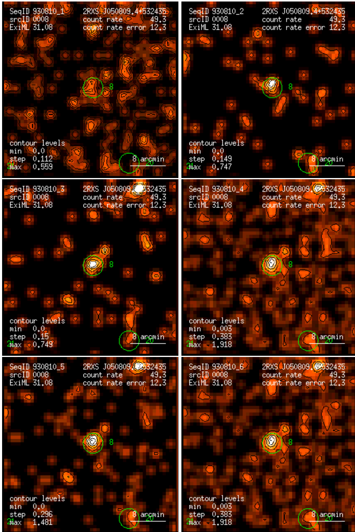
Figure 8: RASS 930810: detection 0008: band rate images, Gaussian filter: (1) PSPC channels 11 – 41, (2) 52 – 90, (3) 91 – 201, (4) 11 – 235, (5) 52 – 201, (6) 11 – 201. Broad band rates in counts/ks. Band rate contour levels in counts/ks/arcmin 2 .
