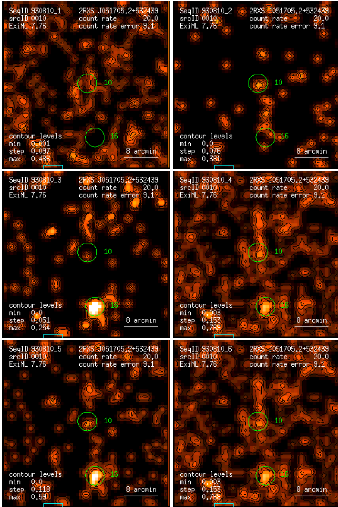
Figure 10: RASS 930810: detection 0010: band rate images, Gaussian filter: (1) PSPC channels 11 – 41, (2) 52 – 90, (3) 91 – 201, (4) 11 – 235, (5) 52 – 201, (6) 11 – 201. Broad band rates in counts/ks. Band rate contour levels in counts/ks/arcmin 2 .
