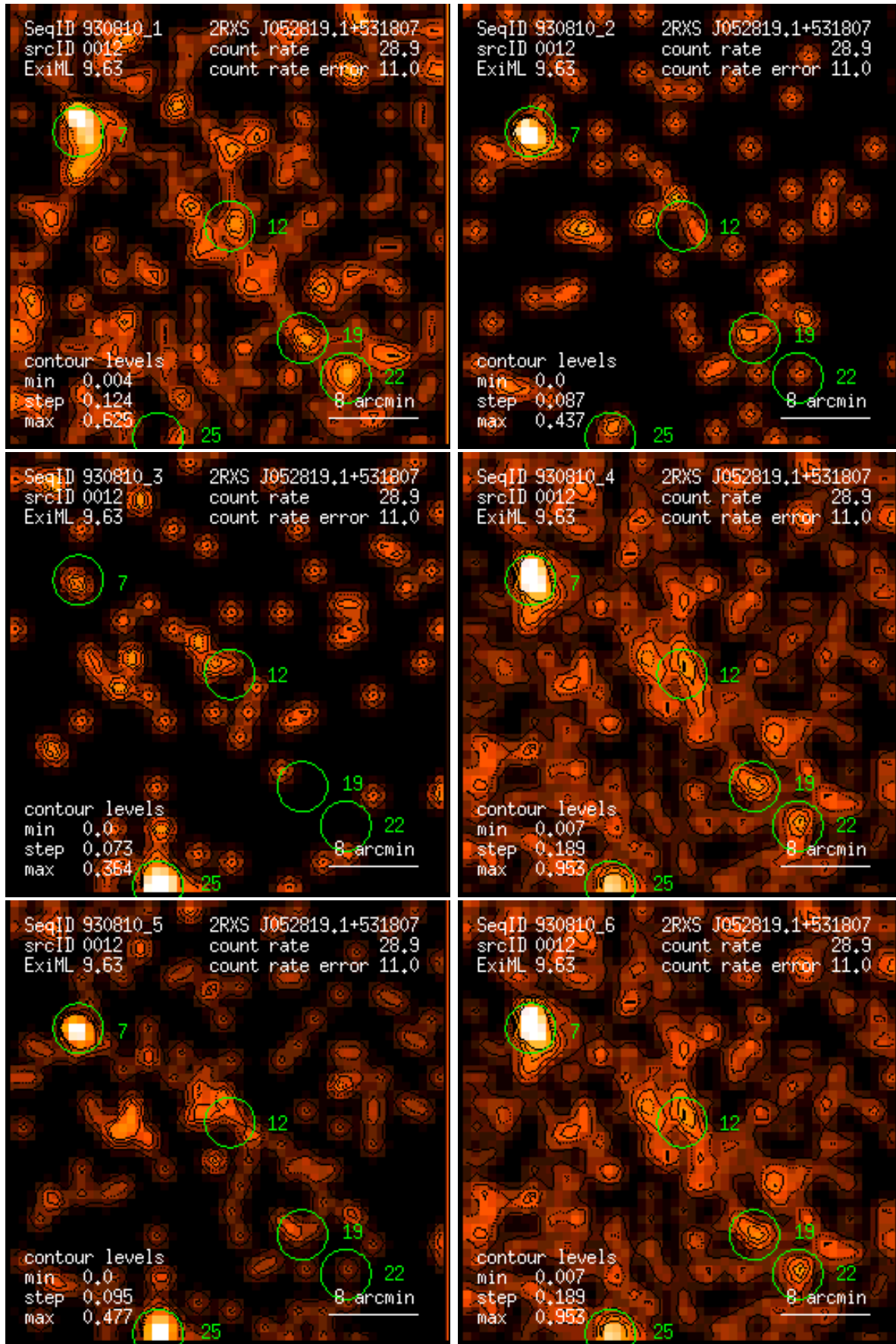
Figure 12: RASS 930810: detection 0012: band rate images, Gaussian filter: (1) PSPC channels 11 – 41, (2) 52 – 90, (3) 91 – 201, (4) 11 – 235, (5) 52 – 201, (6) 11 – 201. Broad band rates in counts/ks. Band rate contour levels in counts/ks/arcmin 2 .
