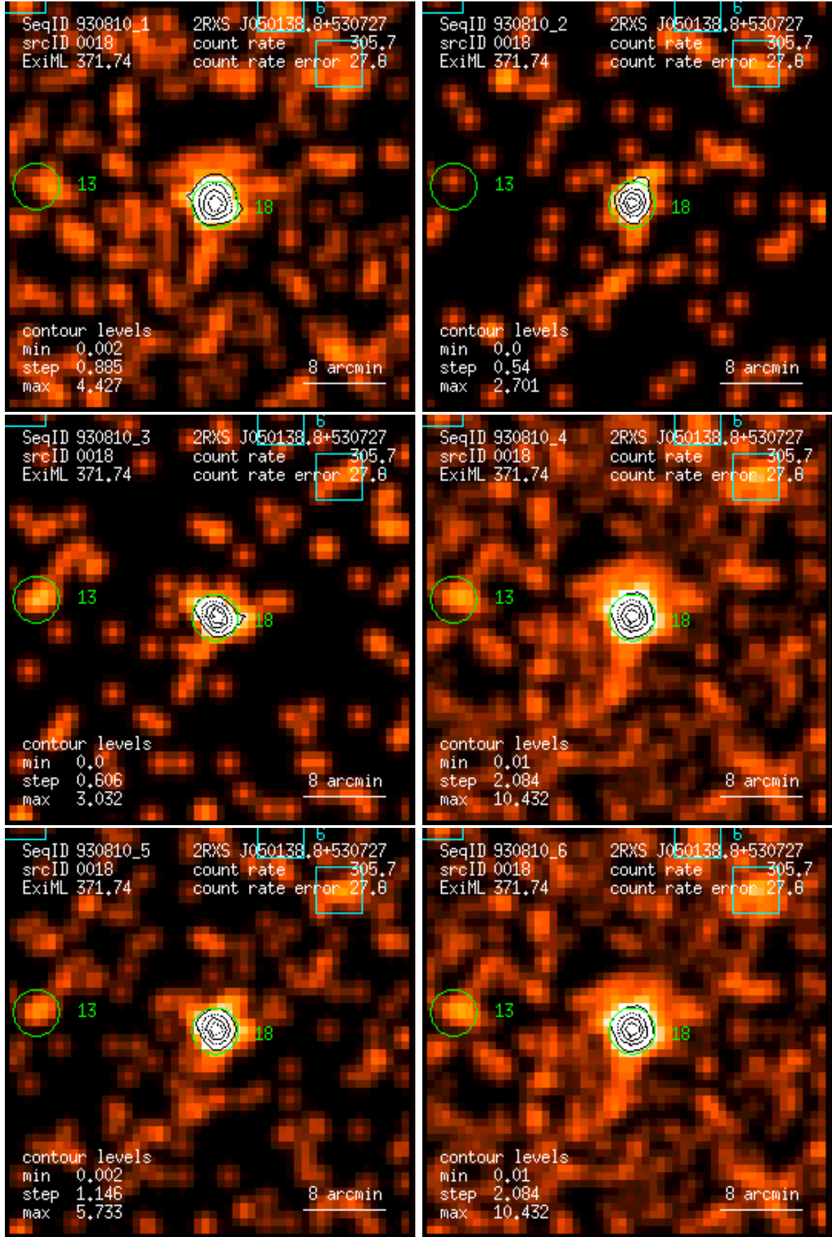
Figure 18: RASS 930810: detection 0018: band rate images, Gaussian filter: (1) PSPC channels 11 – 41, (2) 52 – 90, (3) 91 – 201, (4) 11 – 235, (5) 52 – 201, (6) 11 – 201. Broad band rates in counts/ks. Band rate contour levels in counts/ks/arcmin 2 .
