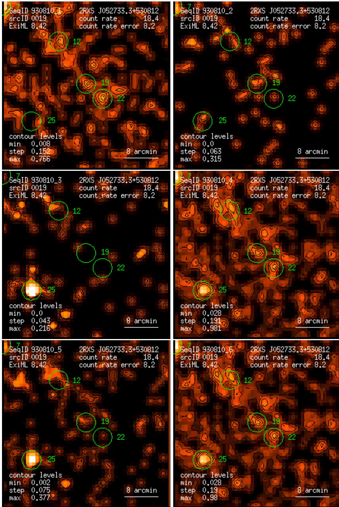
Figure 19: RASS 930810: detection 0019: band rate images, Gaussian filter: (1) PSPC channels 11 – 41, (2) 52 – 90, (3) 91 – 201, (4) 11 – 235, (5) 52 – 201, (6) 11 – 201. Broad band rates in counts/ks. Band rate contour levels in counts/ks/arcmin 2 .
