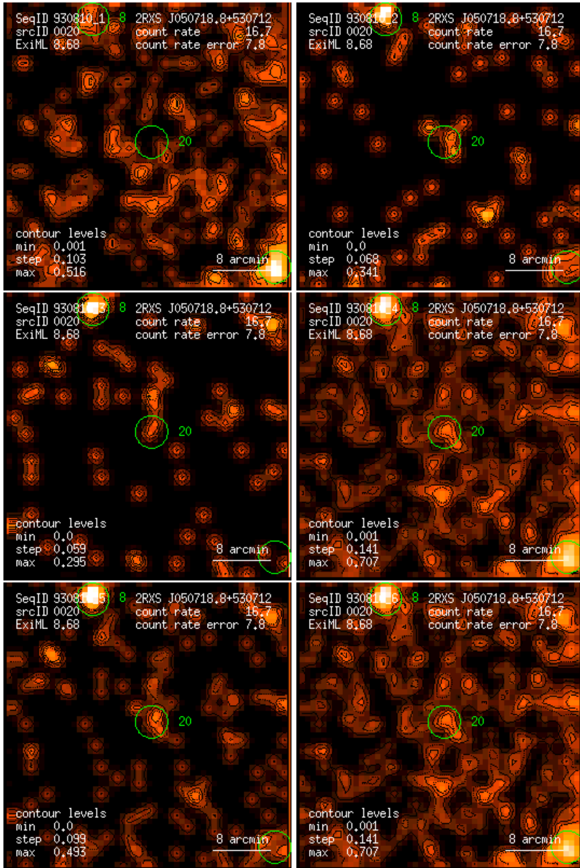
Figure 20: RASS 930810: detection 0020: band rate images, Gaussian filter: (1) PSPC channels 11 – 41, (2) 52 – 90, (3) 91 – 201, (4) 11 – 235, (5) 52 – 201, (6) 11 – 201. Broad band rates in counts/ks. Band rate contour levels in counts/ks/arcmin 2 .
