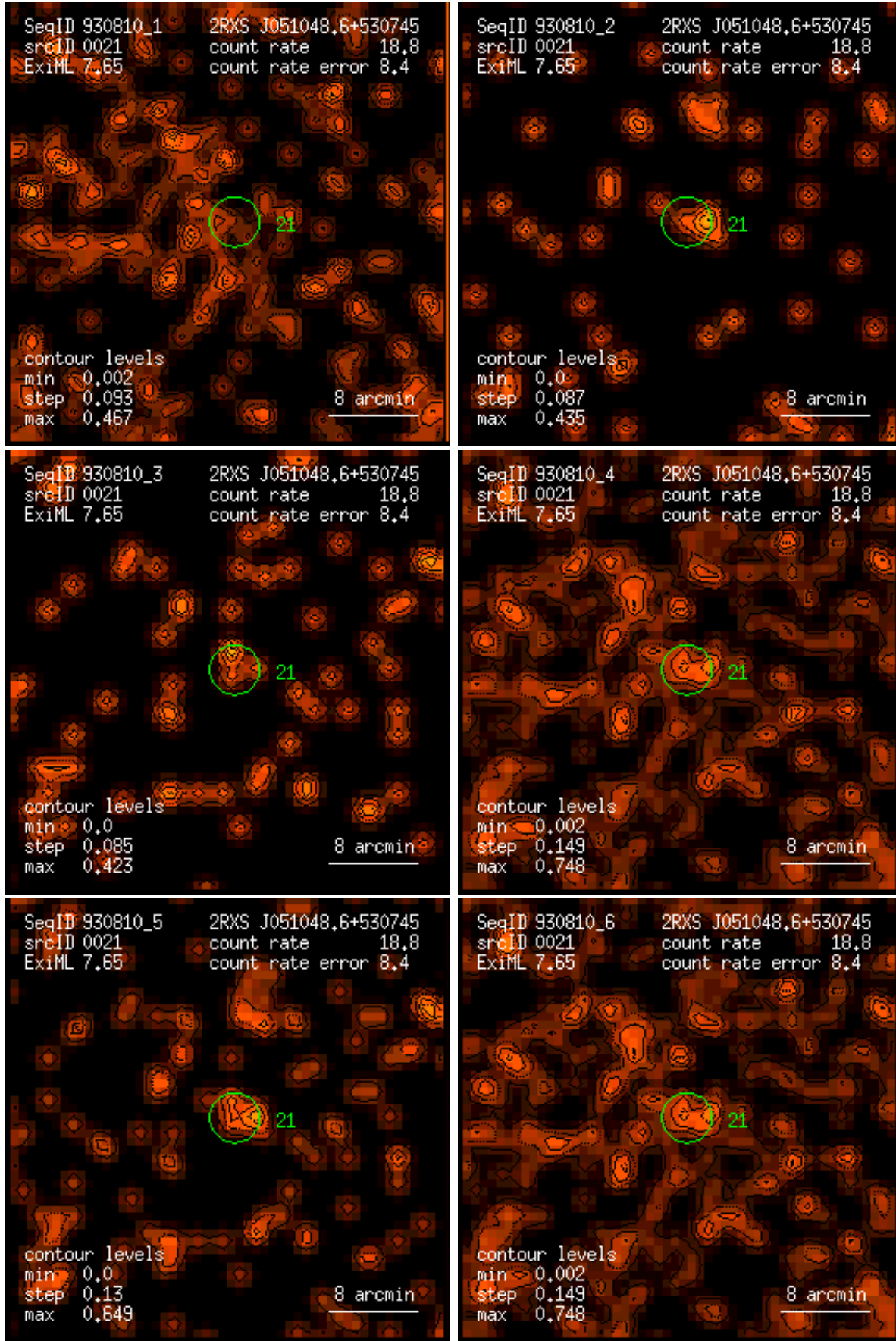
Figure 21: RASS 930810: detection 0021: band rate images, Gaussian filter: (1) PSPC channels 11 – 41, (2) 52 – 90, (3) 91 – 201, (4) 11 – 235, (5) 52 – 201, (6) 11 – 201. Broad band rates in counts/ks. Band rate contour levels in counts/ks/arcmin 2 .
