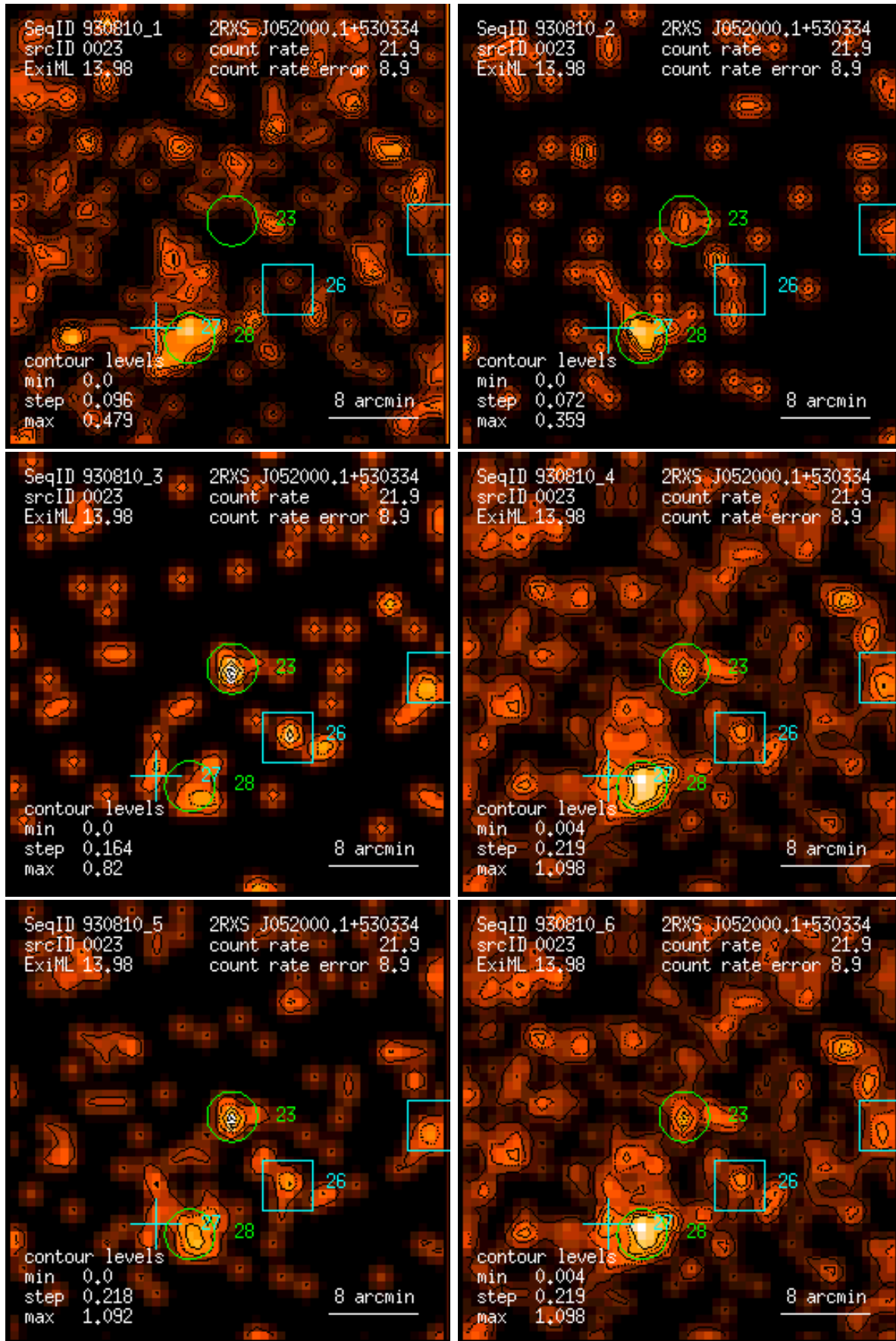
Figure 23: RASS 930810: detection 0023: band rate images, Gaussian filter: (1) PSPC channels 11 – 41, (2) 52 – 90, (3) 91 – 201, (4) 11 – 235, (5) 52 – 201, (6) 11 – 201. Broad band rates in counts/ks. Band rate contour levels in counts/ks/arcmin 2 .
