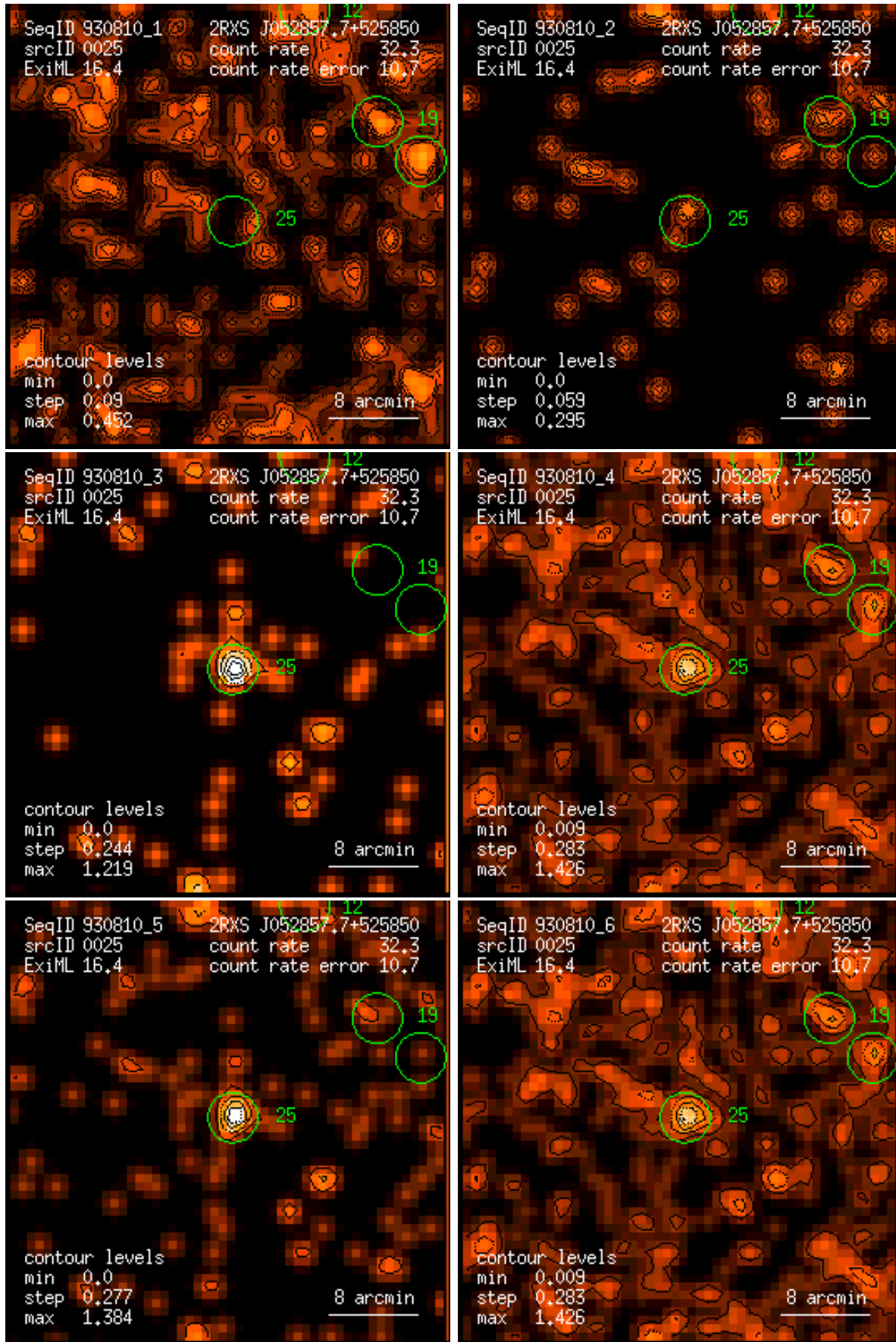
Figure 25: RASS 930810: detection 0025: band rate images, Gaussian filter: (1) PSPC channels 11 – 41, (2) 52 – 90, (3) 91 – 201, (4) 11 – 235, (5) 52 – 201, (6) 11 – 201. Broad band rates in counts/ks. Band rate contour levels in counts/ks/arcmin 2 .
