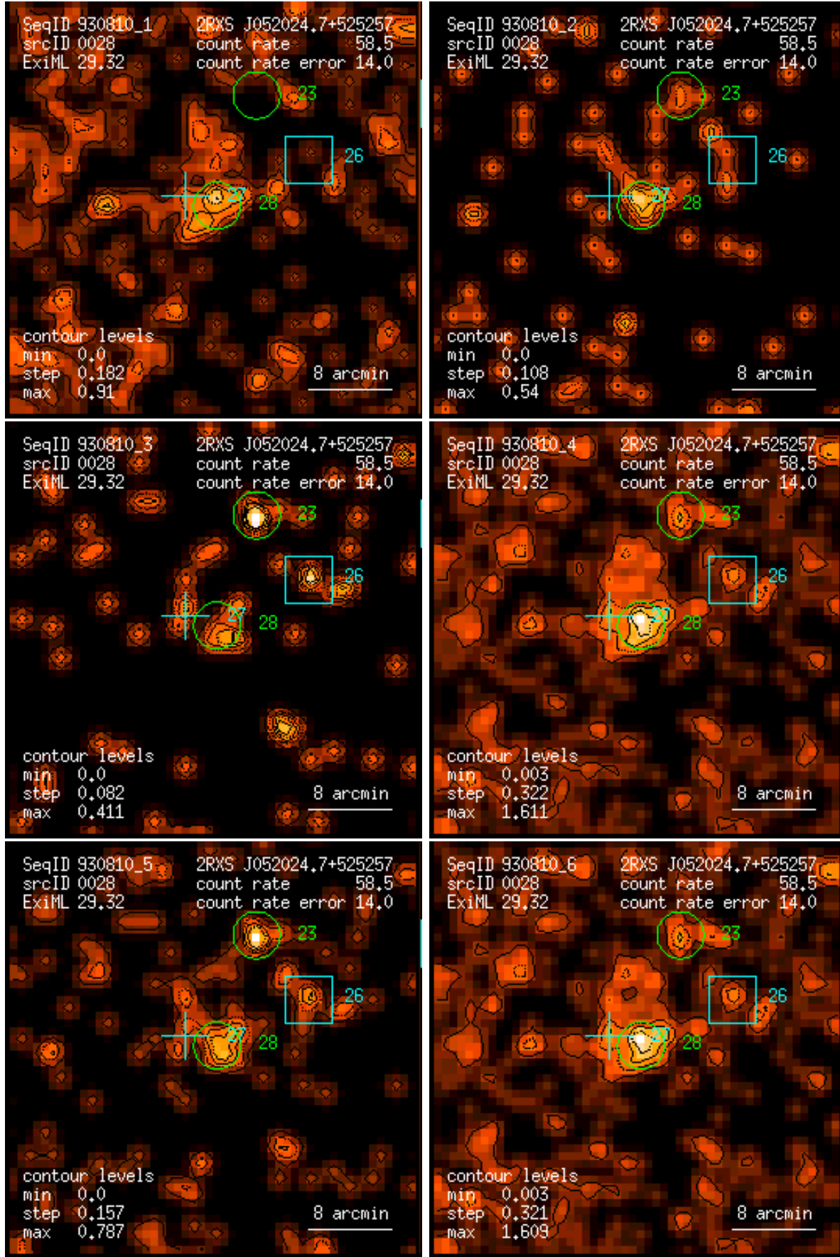
Figure 28: RASS 930810: detection 0028: band rate images, Gaussian filter: (1) PSPC channels 11 – 41, (2) 52 – 90, (3) 91 – 201, (4) 11 – 235, (5) 52 – 201, (6) 11 – 201. Broad band rates in counts/ks. Band rate contour levels in counts/ks/arcmin 2 .
