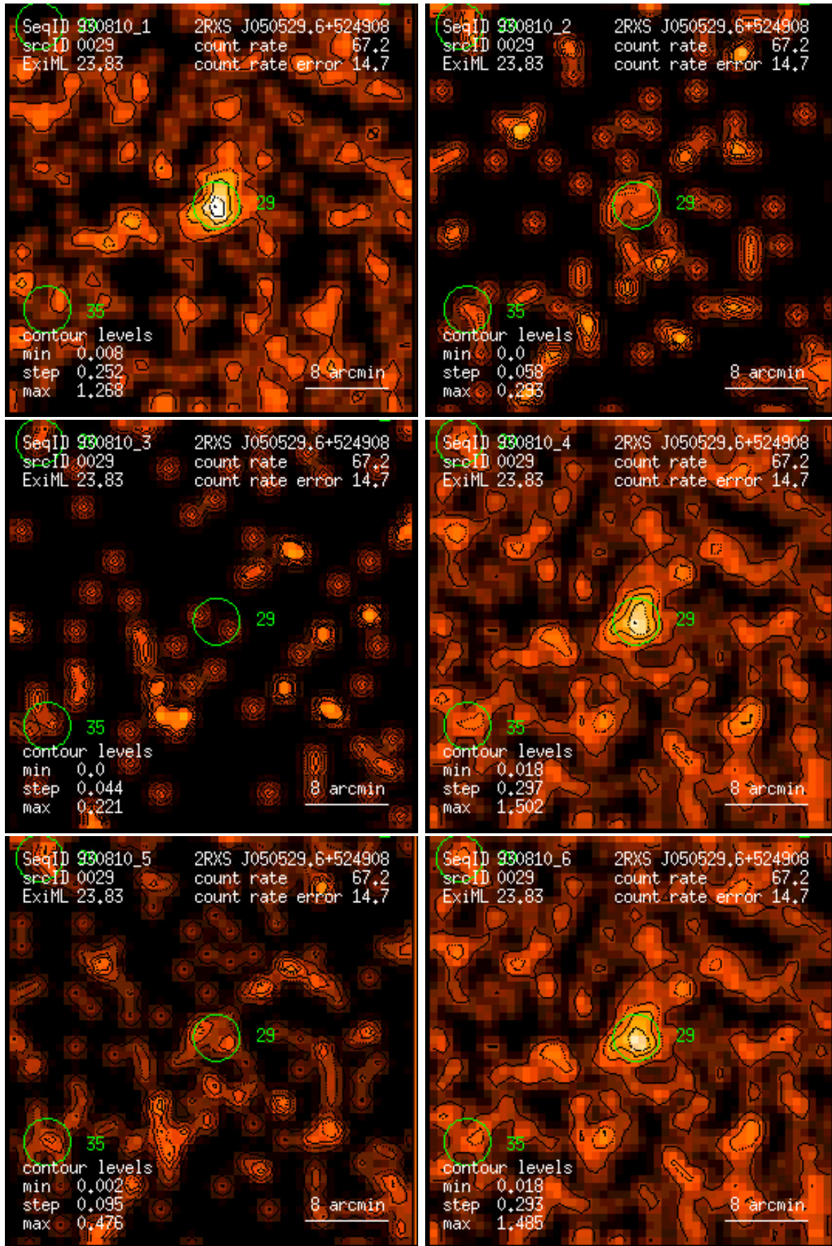
Figure 29: RASS 930810: detection 0029: band rate images, Gaussian filter: (1) PSPC channels 11 – 41, (2) 52 – 90, (3) 91 – 201, (4) 11 – 235, (5) 52 – 201, (6) 11 – 201. Broad band rates in counts/ks. Band rate contour levels in counts/ks/arcmin 2 .
