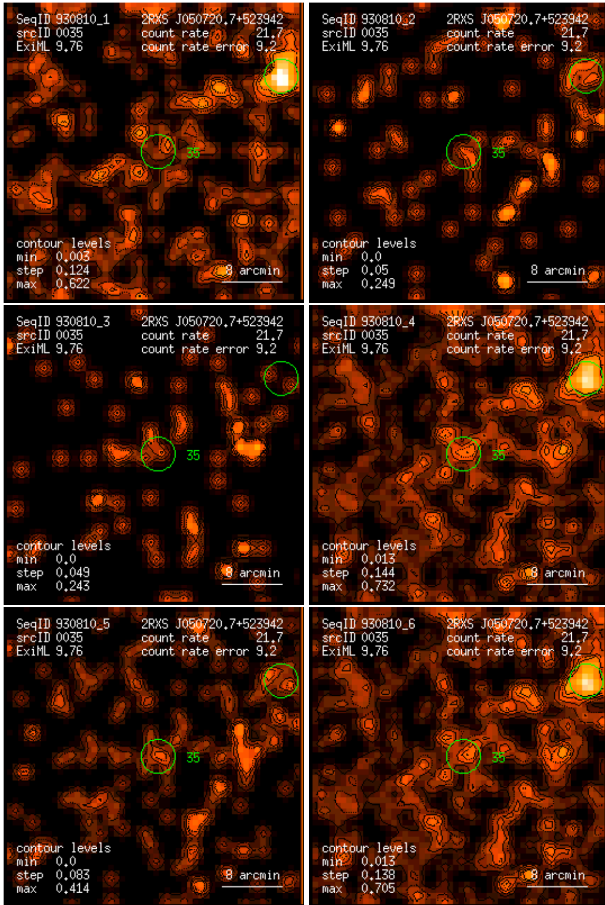
Figure 35: RASS 930810: detection 0035: band rate images, Gaussian filter: (1) PSPC channels 11 – 41, (2) 52 – 90, (3) 91 – 201, (4) 11 – 235, (5) 52 – 201, (6) 11 – 201. Broad band rates in counts/ks. Band rate contour levels in counts/ks/arcmin 2 .
