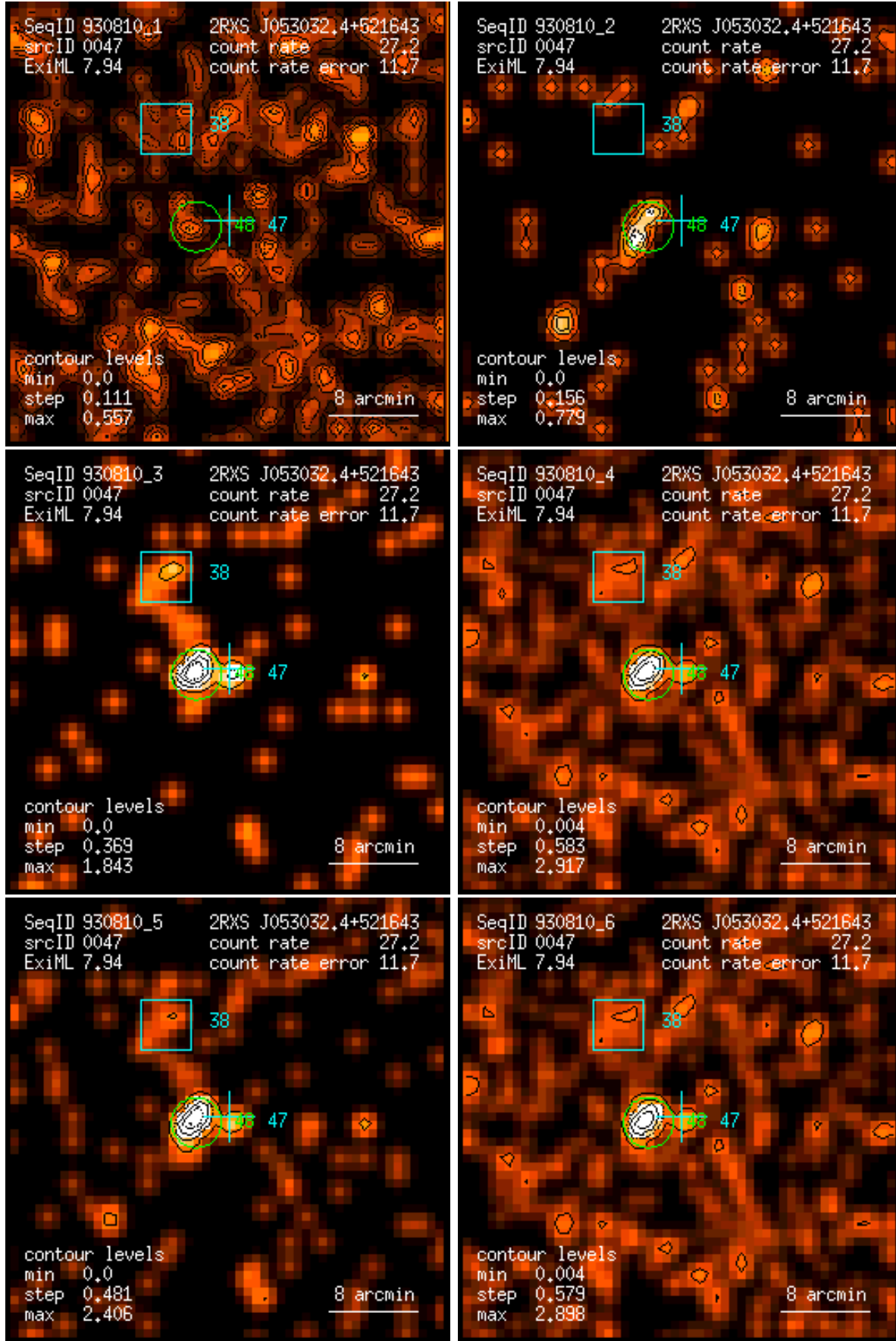
Figure 47: RASS 930810: detection 0047: band rate images, Gaussian filter: (1) PSPC channels 11 – 41, (2) 52 – 90, (3) 91 – 201, (4) 11 – 235, (5) 52 – 201, (6) 11 – 201. Broad band rates in counts/ks. Band rate contour levels in counts/ks/arcmin 2 .
