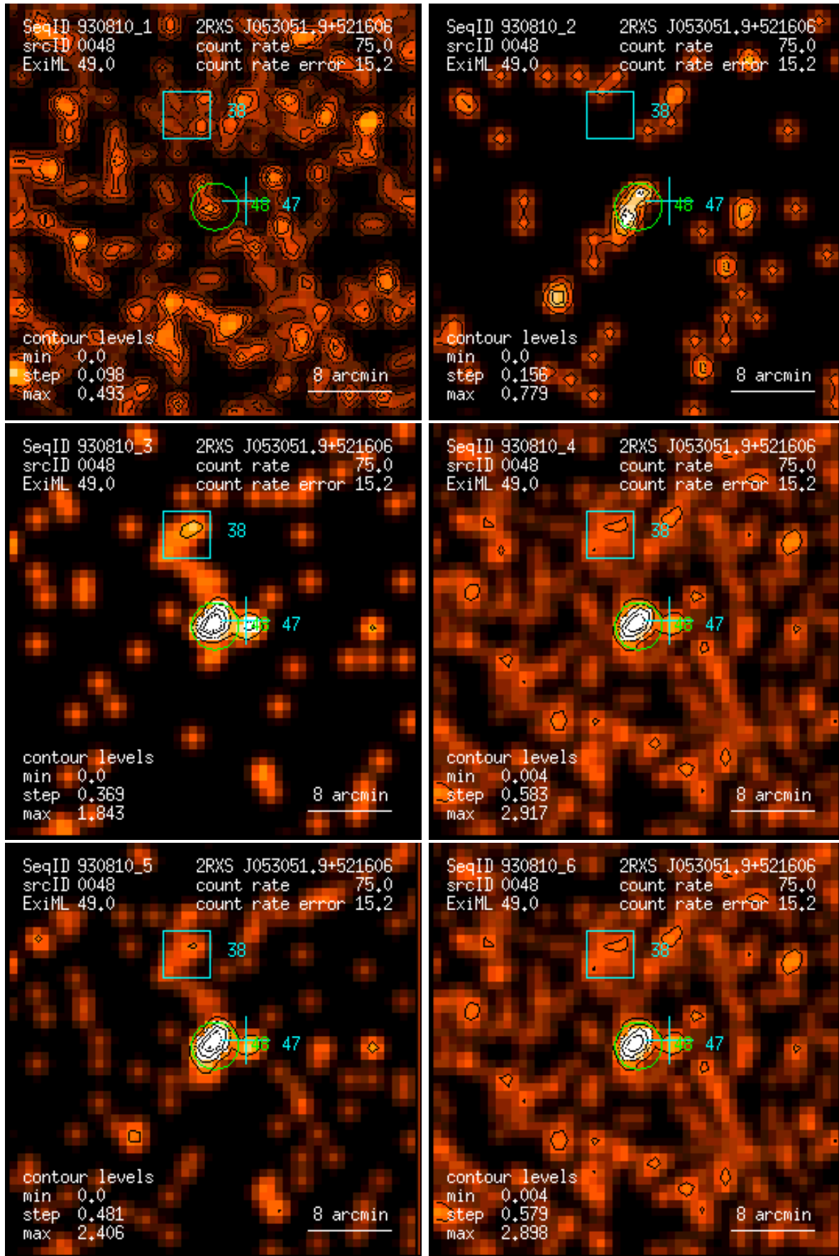
Figure 48: RASS 930810: detection 0048: band rate images, Gaussian filter: (1) PSPC channels 11 – 41, (2) 52 – 90, (3) 91 – 201, (4) 11 – 235, (5) 52 – 201, (6) 11 – 201. Broad band rates in counts/ks. Band rate contour levels in counts/ks/arcmin 2 .
