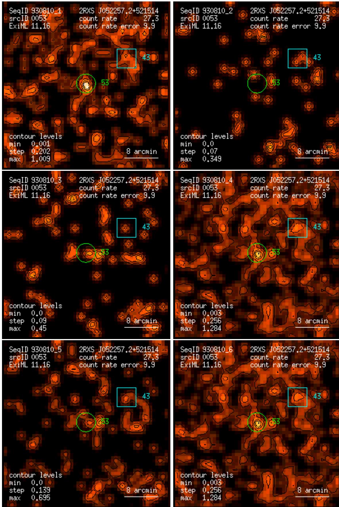
Figure 53: RASS 930810: detection 0053: band rate images, Gaussian filter: (1) PSPC channels 11 – 41, (2) 52 – 90, (3) 91 – 201, (4) 11 – 235, (5) 52 – 201, (6) 11 – 201. Broad band rates in counts/ks. Band rate contour levels in counts/ks/arcmin 2 .
