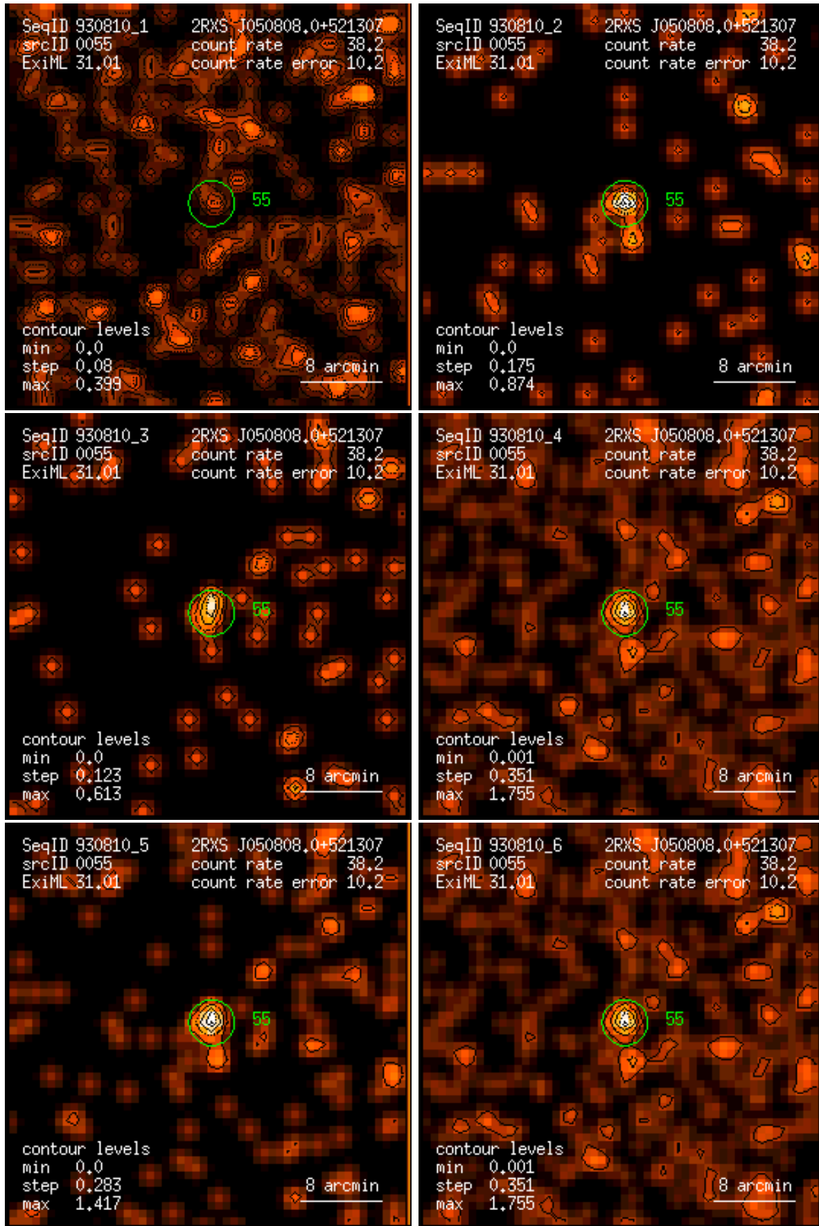
Figure 55: RASS 930810: detection 0055: band rate images, Gaussian filter: (1) PSPC channels 11 – 41, (2) 52 – 90, (3) 91 – 201, (4) 11 – 235, (5) 52 – 201, (6) 11 – 201. Broad band rates in counts/ks. Band rate contour levels in counts/ks/arcmin 2 .
