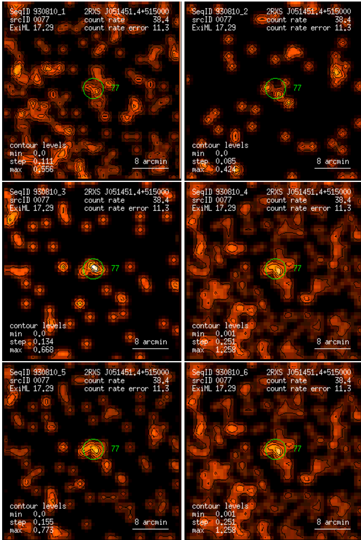
Figure 77: RASS 930810: detection 0077: band rate images, Gaussian filter: (1) PSPC channels 11 – 41, (2) 52 – 90, (3) 91 – 201, (4) 11 – 235, (5) 52 – 201, (6) 11 – 201. Broad band rates in counts/ks. Band rate contour levels in counts/ks/arcmin 2 .
