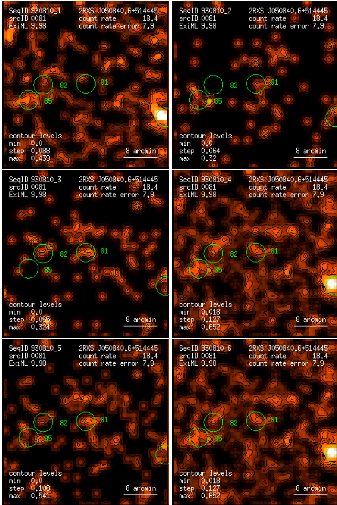
Figure 81: RASS 930810: detection 0081: band rate images, Gaussian filter: (1) PSPC channels 11 – 41, (2) 52 – 90, (3) 91 – 201, (4) 11 – 235, (5) 52 – 201, (6) 11 – 201. Broad band rates in counts/ks. Band rate contour levels in counts/ks/arcmin 2 .
