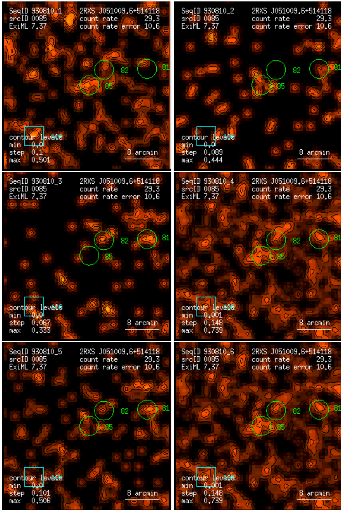
Figure 85: RASS 930810: detection 0085: band rate images, Gaussian filter: (1) PSPC channels 11 – 41, (2) 52 – 90, (3) 91 – 201, (4) 11 – 235, (5) 52 – 201, (6) 11 – 201. Broad band rates in counts/ks. Band rate contour levels in counts/ks/arcmin 2 .
