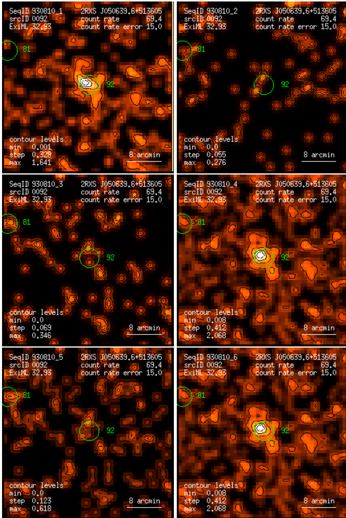
Figure 92: RASS 930810: detection 0092: band rate images, Gaussian filter: (1) PSPC channels 11 – 41, (2) 52 – 90, (3) 91 – 201, (4) 11 – 235, (5) 52 – 201, (6) 11 – 201. Broad band rates in counts/ks. Band rate contour levels in counts/ks/arcmin 2 .
