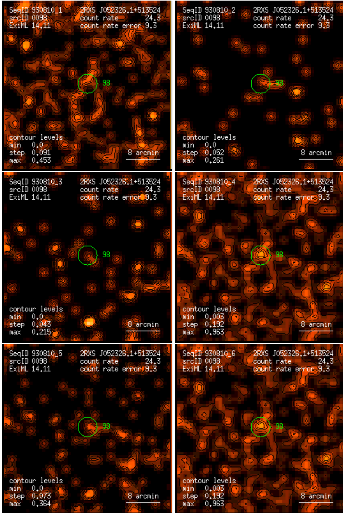
Figure 98: RASS 930810: detection 0098: band rate images, Gaussian filter: (1) PSPC channels 11 – 41, (2) 52 – 90, (3) 91 – 201, (4) 11 – 235, (5) 52 – 201, (6) 11 – 201. Broad band rates in counts/ks. Band rate contour levels in counts/ks/arcmin 2 .
