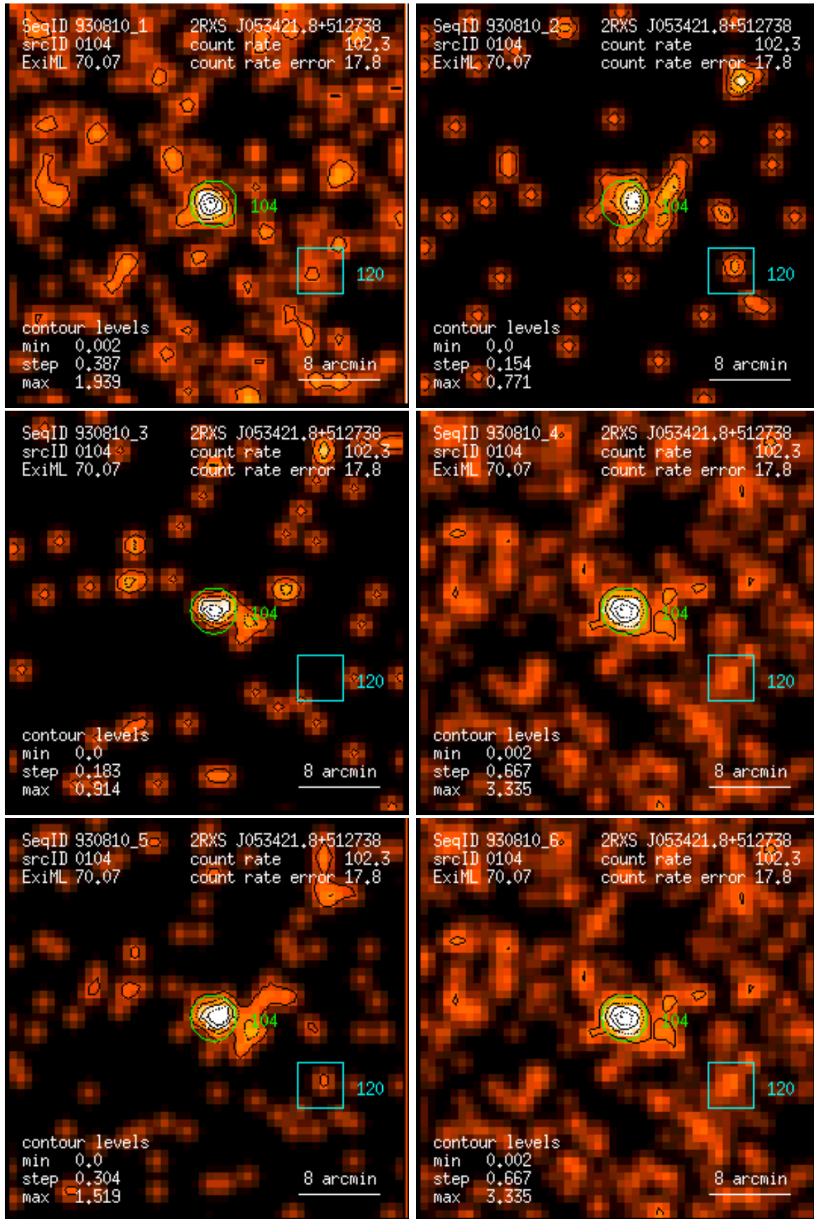
Figure 104: RASS 930810: detection 0104: band rate images, Gaussian filter: (1) PSPC channels 11 – 41, (2) 52 – 90, (3) 91 – 201, (4) 11 – 235, (5) 52 – 201, (6) 11 – 201. Broad band rates in counts/ks. Band rate contour levels in counts/ks/arcmin 2 .
