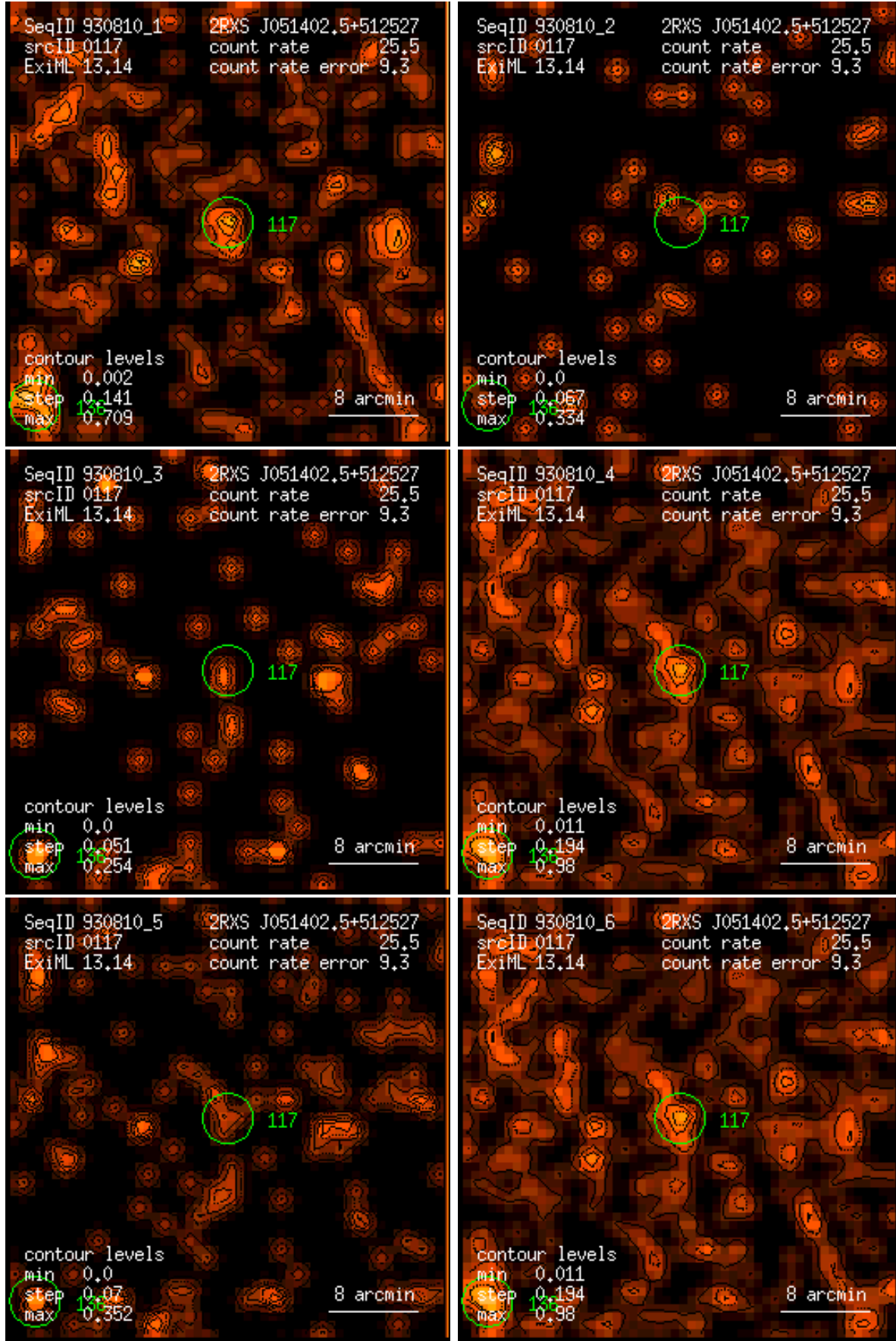
Figure 117: RASS 930810: detection 0117: band rate images, Gaussian filter: (1) PSPC channels 11 – 41, (2) 52 – 90, (3) 91 – 201, (4) 11 – 235, (5) 52 – 201, (6) 11 – 201. Broad band rates in counts/ks. Band rate contour levels in counts/ks/arcmin 2 .
