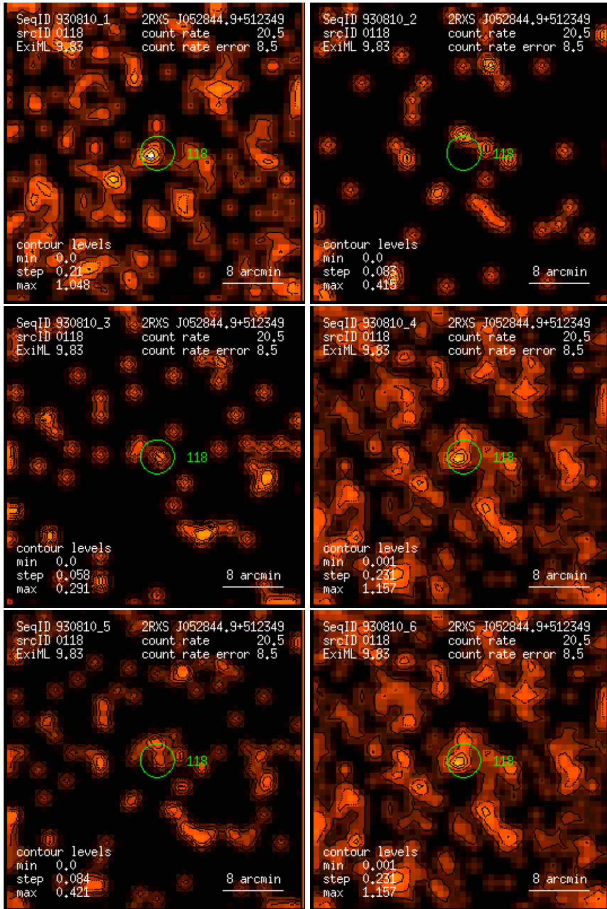
Figure 118: RASS 930810: detection 0118: band rate images, Gaussian filter: (1) PSPC channels 11 – 41, (2) 52 – 90, (3) 91 – 201, (4) 11 – 235, (5) 52 – 201, (6) 11 – 201. Broad band rates in counts/ks. Band rate contour levels in counts/ks/arcmin 2 .
