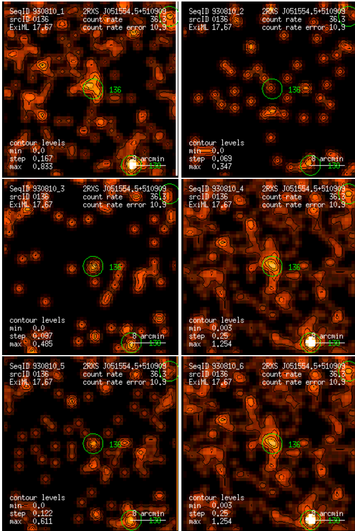
Figure 136: RASS 930810: detection 0136: band rate images, Gaussian filter: (1) PSPC channels 11 – 41, (2) 52 – 90, (3) 91 – 201, (4) 11 – 235, (5) 52 – 201, (6) 11 – 201. Broad band rates in counts/ks. Band rate contour levels in counts/ks/arcmin 2 .
