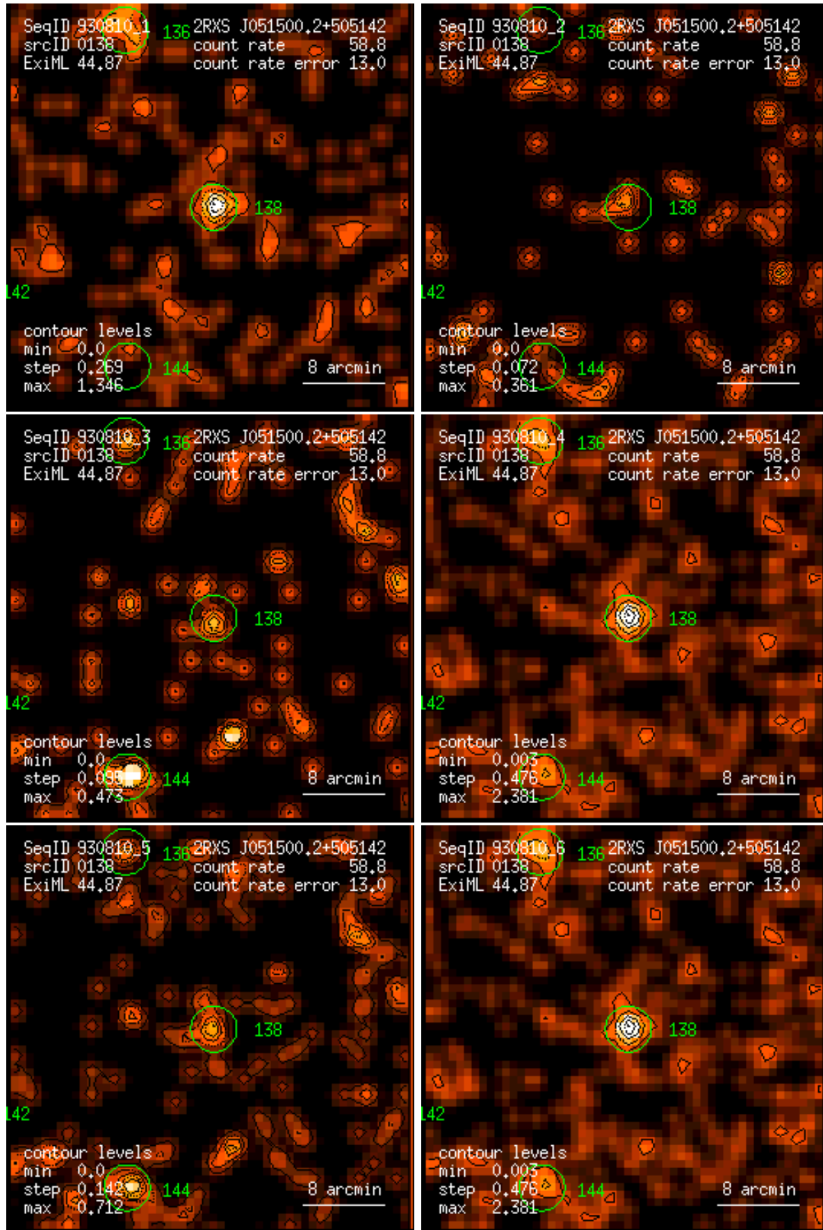
Figure 138: RASS 930810: detection 0138: band rate images, Gaussian filter: (1) PSPC channels 11 – 41, (2) 52 – 90, (3) 91 – 201, (4) 11 – 235, (5) 52 – 201, (6) 11 – 201. Broad band rates in counts/ks. Band rate contour levels in counts/ks/arcmin 2 .
