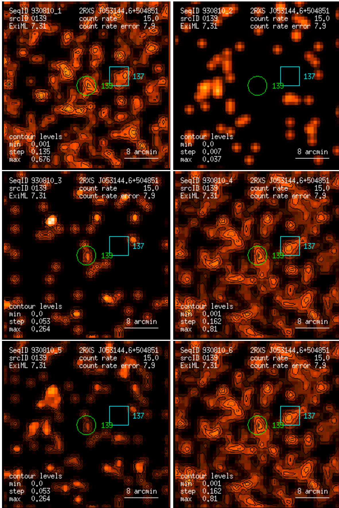
Figure 139: RASS 930810: detection 0139: band rate images, Gaussian filter: (1) PSPC channels 11 – 41, (2) 52 – 90, (3) 91 – 201, (4) 11 – 235, (5) 52 – 201, (6) 11 – 201. Broad band rates in counts/ks. Band rate contour levels in counts/ks/arcmin 2 .
