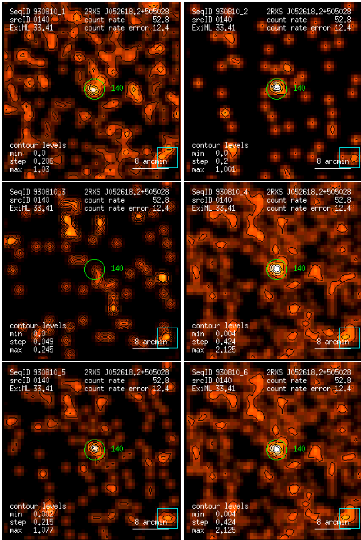
Figure 140: RASS 930810: detection 0140: band rate images, Gaussian filter: (1) PSPC channels 11 – 41, (2) 52 – 90, (3) 91 – 201, (4) 11 – 235, (5) 52 – 201, (6) 11 – 201. Broad band rates in counts/ks. Band rate contour levels in counts/ks/arcmin 2 .
