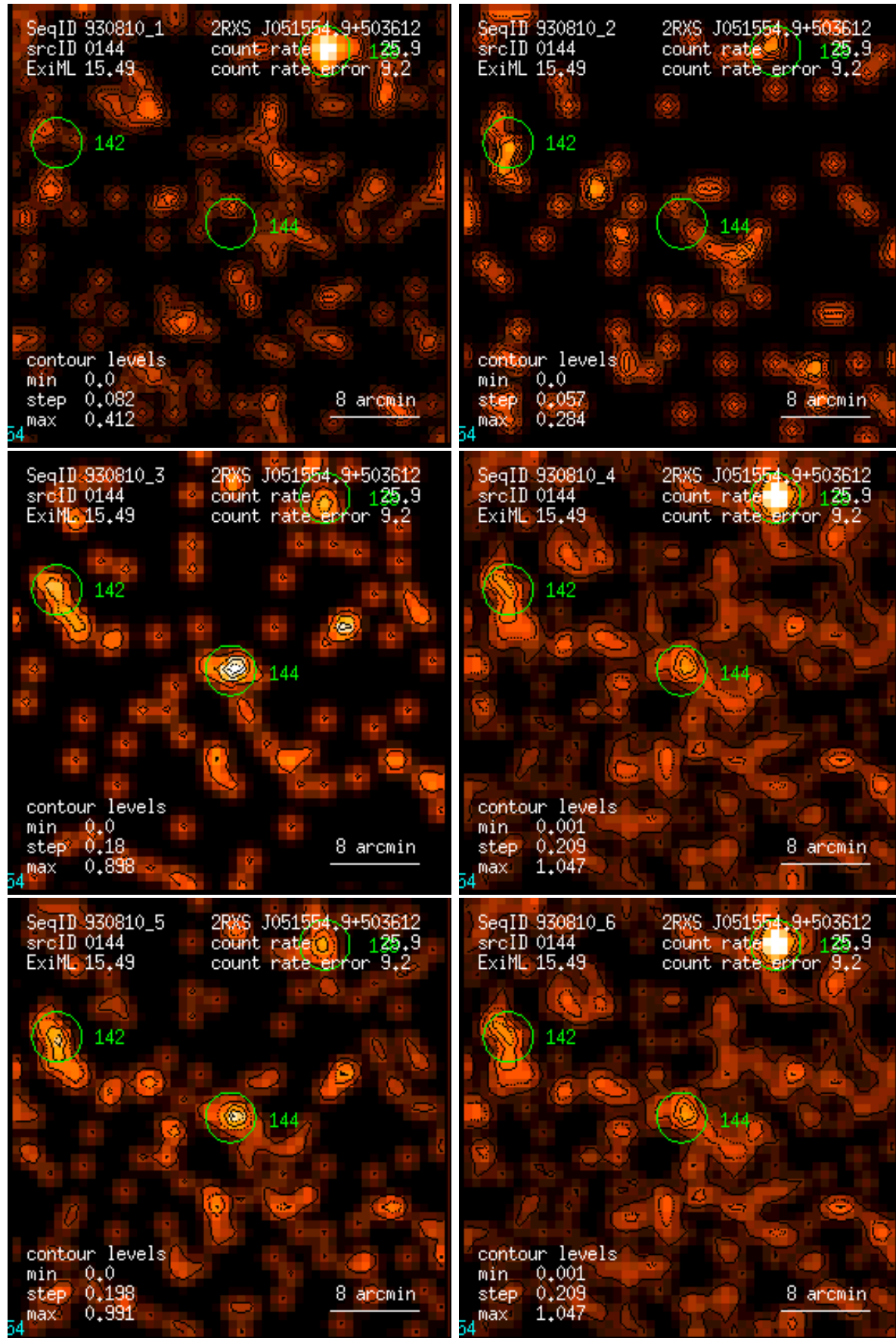
Figure 144: RASS 930810: detection 0144: band rate images, Gaussian filter: (1) PSPC channels 11 – 41, (2) 52 – 90, (3) 91 – 201, (4) 11 – 235, (5) 52 – 201, (6) 11 – 201. Broad band rates in counts/ks. Band rate contour levels in counts/ks/arcmin 2 .
