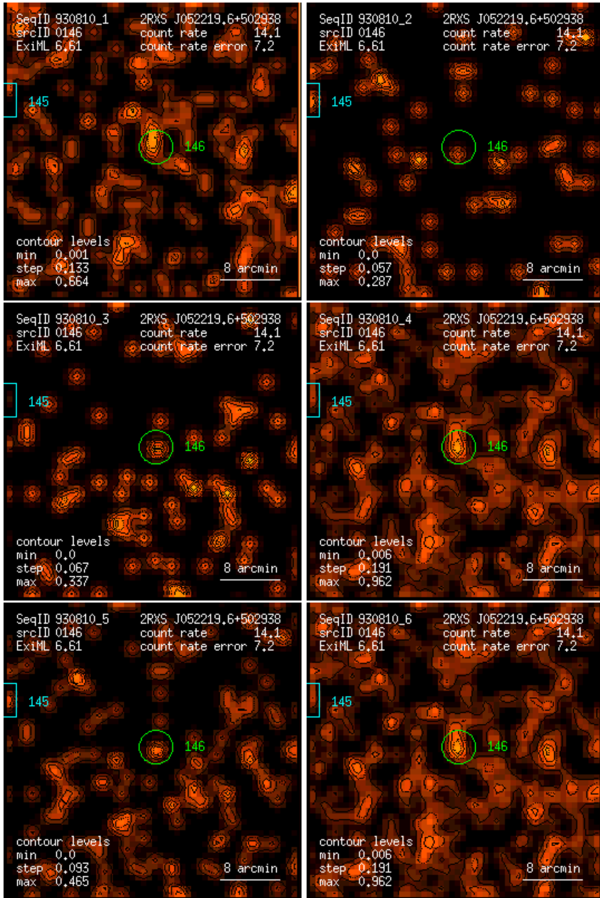
Figure 146: RASS 930810: detection 0146: band rate images, Gaussian filter: (1) PSPC channels 11 – 41, (2) 52 – 90, (3) 91 – 201, (4) 11 – 235, (5) 52 – 201, (6) 11 – 201. Broad band rates in counts/ks. Band rate contour levels in counts/ks/arcmin 2 .
