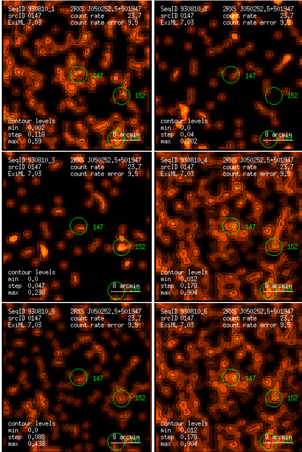
Figure 147: RASS 930810: detection 0147: band rate images, Gaussian filter: (1) PSPC channels 11 – 41, (2) 52 – 90, (3) 91 – 201, (4) 11 – 235, (5) 52 – 201, (6) 11 – 201. Broad band rates in counts/ks. Band rate contour levels in counts/ks/arcmin 2 .
